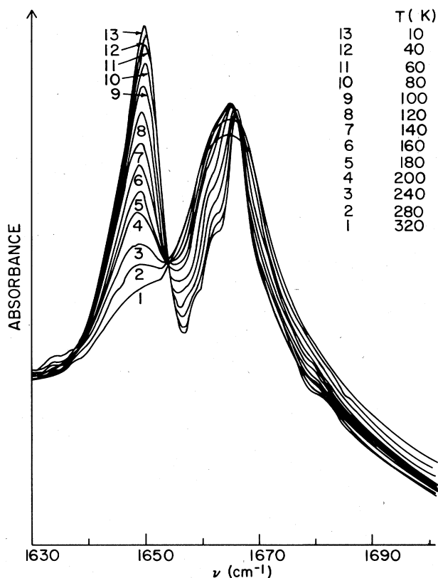
FIG. 5. ir-absorption spectra of ACN microcrystals in KBr in the region of the amide I mode. Results of 100 scans on a Nicolet model no. 7000 FTIR at 0.5 \text{ cm}^{-1} resolution.
