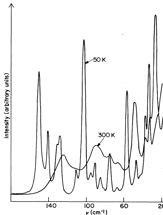
FIG. 14. Raman spectra of the low-frequency modes at 300 and 50 K.
