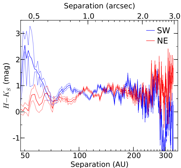
Figure 9. Disk H-K_s color (solid lines) relative to the star as a function of radius, computed from self-subtraction-corrected one-dimensional brightness measurements. The SW ansa is in blue and the NE is in red. Dashed lines show the 1\sigma confidence intervals, which include \chi^2_\nu scaling and uncertainties associated with our simplified disk model. The disk is generally red, and its color is approximately constant with r . We have lower confidence in our measurements at r \gtrsim 160 AU because of the low S/N in K_s in that region.
