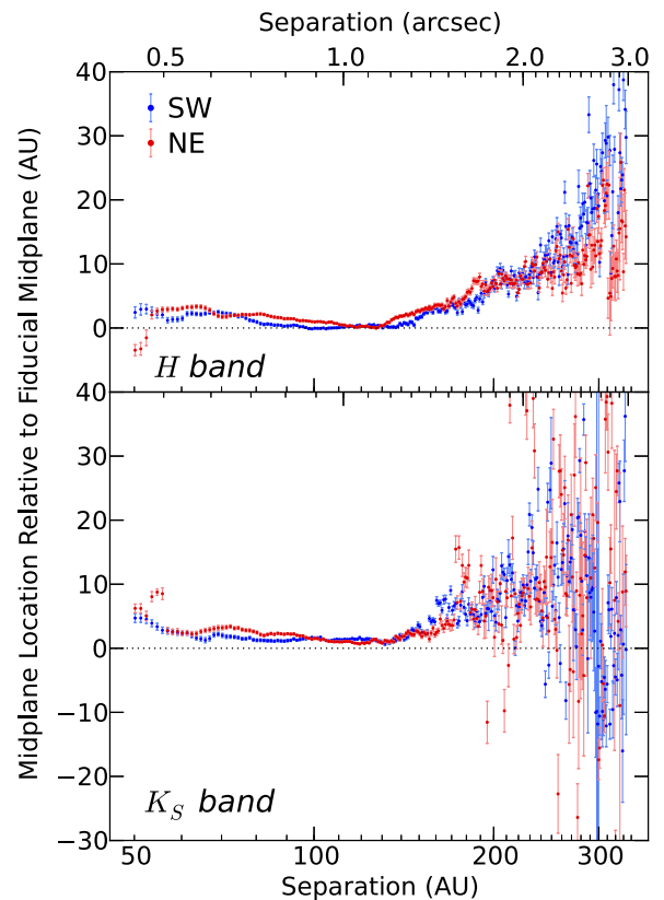
Figure 8. Disk midplane location measured by the self-subtraction modeling algorithm and relative to the fiducial midplane location (PA = 47.5^\circ east of north; dotted line) as a function of separation for SW and NE ansae in H and K_s . A positive location corresponds to a position northwest of the fiducial midplane as it extends from the star, and a negative location is southeast of the fiducial midplane. The profiles show considerable northwest curvature of the disk, particularly in H . The error bars represent 1\sigma uncertainty levels that include \chi^2_v scaling and uncertainties associated with our simplified disk model. (A color version of this figure is available in the online journal.)
