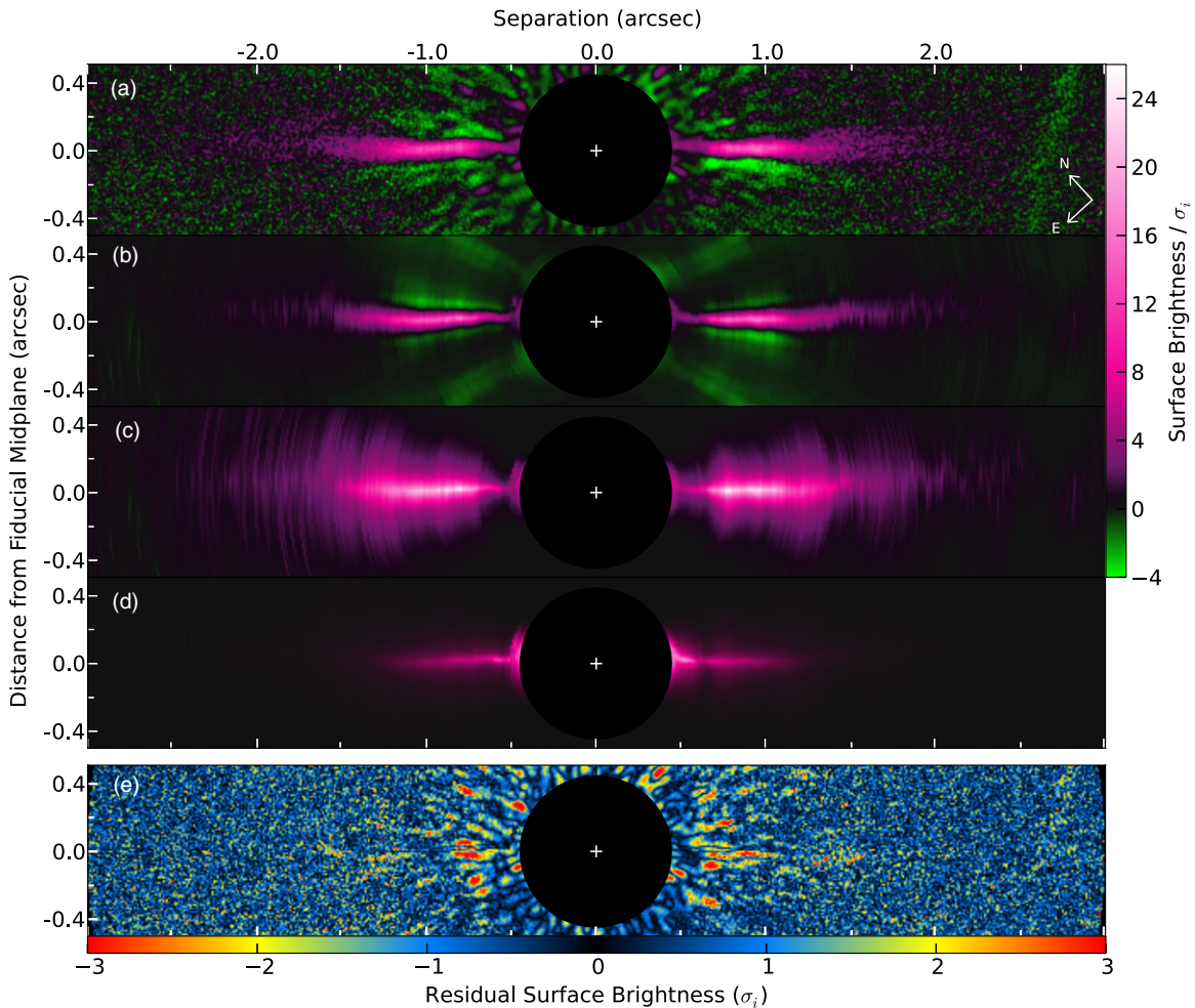
Figure 5. K_s images of the disk surface brightness directly analogous to the H images in Figure 4. The brightness scale for panel (d) is the same as in H , but the scale for panels (a)–(c) is slightly different than in H to better show the disk features.
