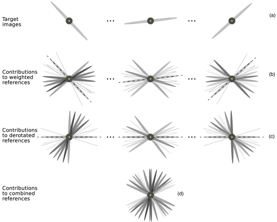
Figure 1. Illustration of the reference-image selection and combination process used in LOCI and our self-subtraction model. Ellipses represent edge-on disks arranged at various P.A.’s according to the parallactic rotation in a synthetic data set, while the dark gray circle is centered on the star and masks the region inside of a coronagraph’s inner working angle. The gray level of an ellipse indicates the weight of that image in the reference PSF combination as determined by the c_{ij}(r) coefficient (darker means more heavily weighted). In row (a), the disks of the target images T_i(r, \theta) are positioned at their associated \theta_i . In row (b), the disks of the reference images T_j(r, \theta) are weighted by their c_{ij} and summed to create the reference PSF for T_i . The disk of the target image and disks located within the minimum rotation threshold for a given separation r (marked by solid lines and white fill) have c_{ij}(r) = 0 and do not contribute to the reference PSF. Note that the amount of P.A. rotation is exaggerated in this diagram for clarity, leading to fewer disks with c_{ij}(r) = 0 than in a typical real data set. In row (c), all reference PSFs from row (b) are derotated so that the midplane of the target image’s disk lies at \theta = 0^\circ . In row (d), all reference PSFs from row (c) are aligned to the star and summed to create the self-subtraction function for the final LOCI-processed image at separation r .
