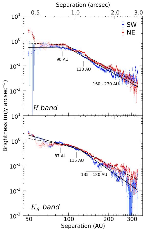
Figure 6. One-dimensional integrated brightness profiles produced by our self-subtraction modeling process in H and K_s . Measurements represent the disk brightness before flux loss caused by ADI/LOCI processing. The SW ansa is in blue and the NE is in red. Locations of significant asymmetries are labeled. The error bars represent 1\sigma uncertainty levels that include \chi^2 scaling and uncertainties associated with our simplified disk model, with the caveat that the errors may remain underestimated as a result of overconstrained least-squares fit parameters. The best-fit power-law functions are shown as solid lines for the SW and as dashed lines for the NE. Breaks in the power laws occur at r \approx 95\text{--}125 AU. Low S/N in the K_s data reduces the reliability of measurements at r \gtrsim 160 AU.
