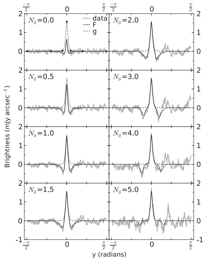
Figure 3. Examples of one-dimensional semiannuli fitted by our self-subtraction modeling algorithm. The different panels show semiannuli from the H -band images reduced using different N_\delta -values, but all from the SW ansa at r = 133 AU. The thick gray lines represent the data, the solid black line is the self-subtracted model ( F ) fit to the data, and the dashed line is the best-fit cubic spline model of the underlying disk vertical brightness profile ( g ), with filled circles marking the control-point locations in the first panel. The scene g is constant in all panels, but the self-subtracted model differs according to N_\delta .
