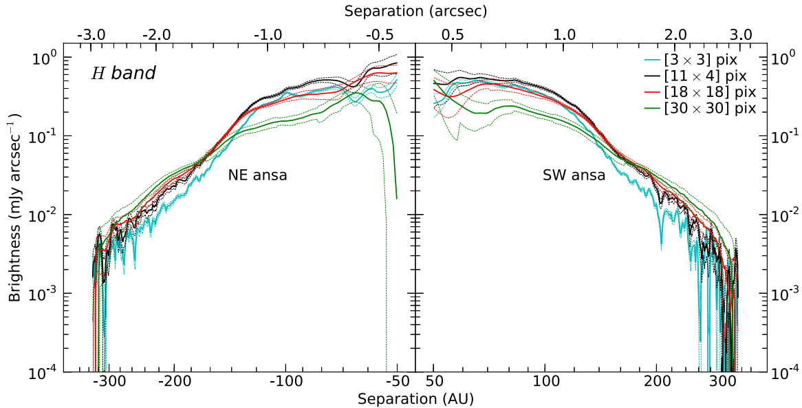
Figure 10. Aperture photometry brightness measurements converted to one-dimensional integrated brightness profiles (solid lines) for the H -band LOCI final image. Dashed lines show the 1\sigma confidence intervals. Four different aperture sizes (azimuthal \times radial diameter) were used: 3 \times 3 (cyan), 11 \times 4 (black), 18 \times 18 (red), and 30 \times 30 pixels (green). Brightness values for a given separation can vary between different-sized apertures by factors up to \sim 2.5 . The star is located at x = 0 (not plotted).
