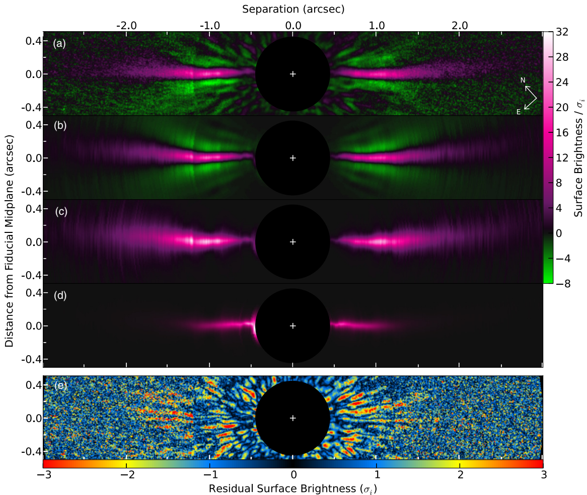
Figure 4. H -band images of the disk surface brightness. All panels except (d) have been scaled by \sigma_i , which is the separation-dependent random error in the data at each pixel i (not to be confused with \sigma calculated from a \chi^2 -scaled covariance matrix). (a) LOCI-processed image from Figure 2, derotated by 42.5^\circ so that the fiducial midplane lies along the horizontal. (b) Model of the self-subtracted disk produced by subtracting the forward-modeled self-subtraction function from the best-fit model of the disk’s underlying brightness distribution. Negative-brightness regions above and below the midplane match those in the real data. (c) Best-fit model of the disk’s underlying brightness distribution absent of self-subtraction. Disk curvature toward the northwest is clearly visible. (d) Same as panel (c), except the brightness is not scaled by \sigma_i and follows a linear color stretch from 0 to 13 mJy arcsec ^{-2} . (e) Deviate map for panels (a)–(c) normalized by \sigma_i . Note that the deviates were not scaled by \chi_i^2 and thus do not account for correlated pixels or overconstrained model parameters.
