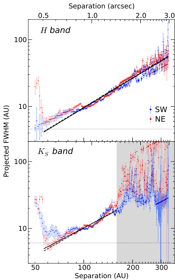
Figure 7. Projected FWHM of the pre-self-subtraction model disk as a function of separation for SW and NE ansae in H and K_s . We find the FWHM to generally increase with separation. The best-fit power-law functions are shown as solid lines for the SW and as dashed lines for the NE. The gray-shaded area in K_s marks the low-confidence region that we exclude from most of our results and discussion. The horizontal, dotted line indicates the diffraction limit ( 1.22\lambda/D ) at each band’s central wavelength. The error bars represent 1\sigma uncertainty levels that include \chi^2_v scaling and uncertainties associated with our simplified disk model.
