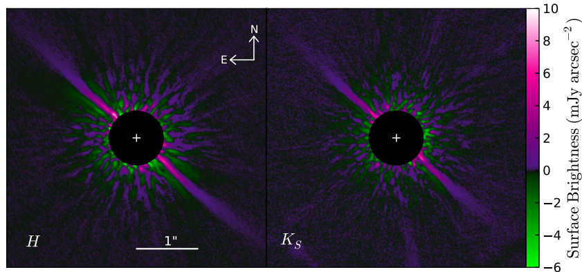
Figure 2. Final LOCI-processed images of the disk surface brightness in scattered light in H (left) and K_s (right) bands. The disk is seen approximately edge-on with one ansa to the NE and the other to the SW of the star. Green areas are negative-brightness regions created by self-subtraction or imperfect PSF subtraction. The star’s location is marked by a white cross. The black circle masks the innermost radii, where either residual speckle noise dominates or the coronagraph mask obscures the disk.
