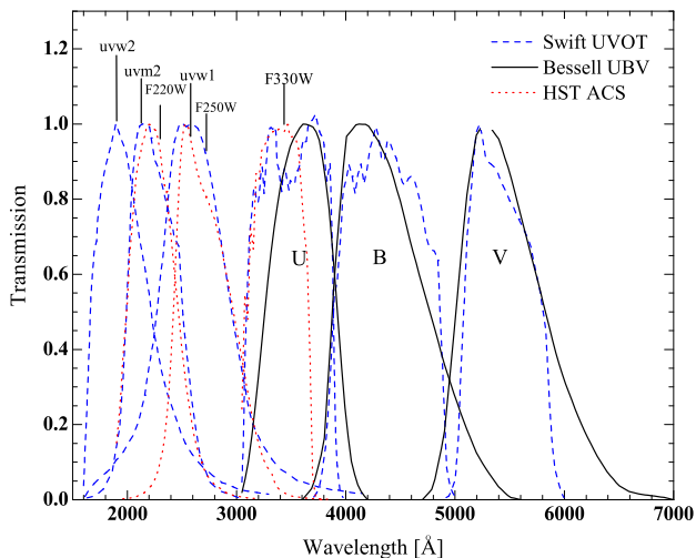
FIG. 6.— Comparison of transmission curves of Swift UVOT filters with HST ACS in the UV and with the Johnson system in UBV .
