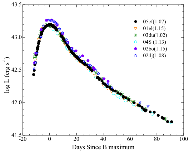
FIG. 24.— The uvoir bolometric light curve of SN 2005cf. Overplotted are the corresponding light curves of the comparison SNe Ia. The number in parentheses represent the \Delta m_{15} values for the SNe Ia.
