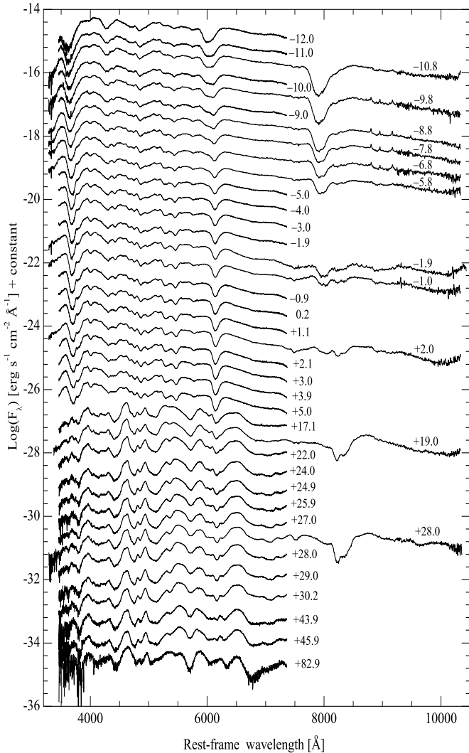
FIG. 16.— Optical spectral evolution of SN 2005cf. The spectra have been corrected for the redshift of the host galaxy ( v_{\text{hel}} = 1967 km s ^{-1} ) but not reddening, and they have been shifted vertically by arbitrary amounts for clarity. The numbers on the right-hand side mark the epochs of the spectra in days after B maximum.
