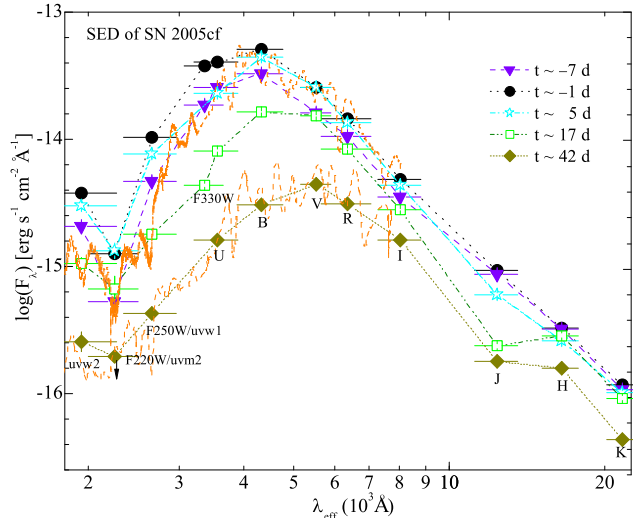
FIG. 12.— The spectral energy distribution evolution of SN 2005cf at t = -7 , -1 , +5 , +17 , and +42 d after the B -band maximum. The photometric points are shown with error bars (vertical ones for uncertainties and horizontal ones for the FWHM of the filters). Overlaid are the HST FOS spectra of SN 1992A (dotted curves) from Kirshner et al. (1993), obtained at t \approx +5 d and +45 d, respectively. Note that the error bar of the flux is in most cases smaller than the size of the symbol.
