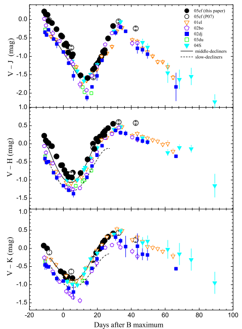
FIG. 14.— The V - JHK color curves of SN 2005cf, together with those of SNe 2001el, 2002bo, 2002dj, 2003du, and 2004S. The dashed lines represent the mean loci of the unreddened SNe Ia with \Delta m_{15} = 0.8 - 1.0 mag; the solid lines denote those with \Delta m_{15} = 1.0 - 1.3 mag (Krisciunas et al. 2004a).
