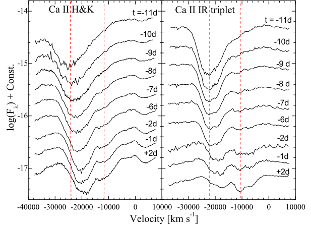
FIG. 21.— Premaximum evolution in velocity space for the Ca II H&K and NIR triplet of SN 2005cf. Vertical dashed lines indicate, respectively, the highest velocity in the earliest phase ( \sim 23000 \text{ km s}^{-1} ) and the photospheric velocity (at \sim 11000 \text{ km s}^{-1} ).
