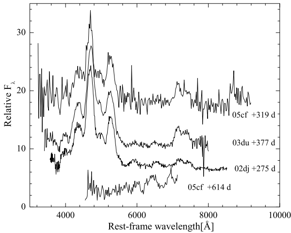
FIG. 18.— Late-time nebular spectra of SN 2005cf, slightly smoothed. The nebular spectra of SN 2003du (Stanishev et al. 2007) and SN 2002dj (Pignata et al. 2008) at about the same phase as the earlier SN 2005cf spectrum are shown for comparison. Both reddening and redshift corrections have been applied to the spectra.
