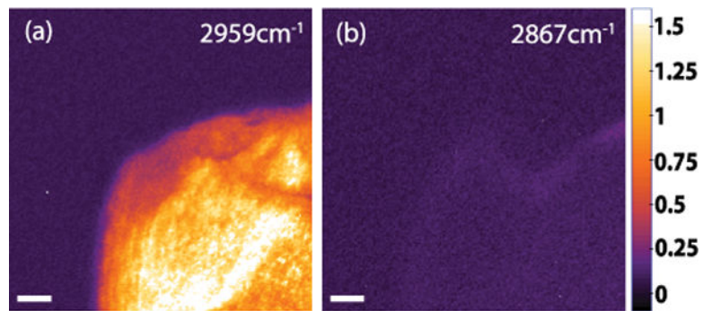
Fig. 4. (Color online) Spectral scan images of collagen with the VR-SFG microscope. SFG images at (a) on-resonance, 2959 cm -1 , and (b) off-resonance, 2867 cm -1 . The scale bar is 20 μm.
