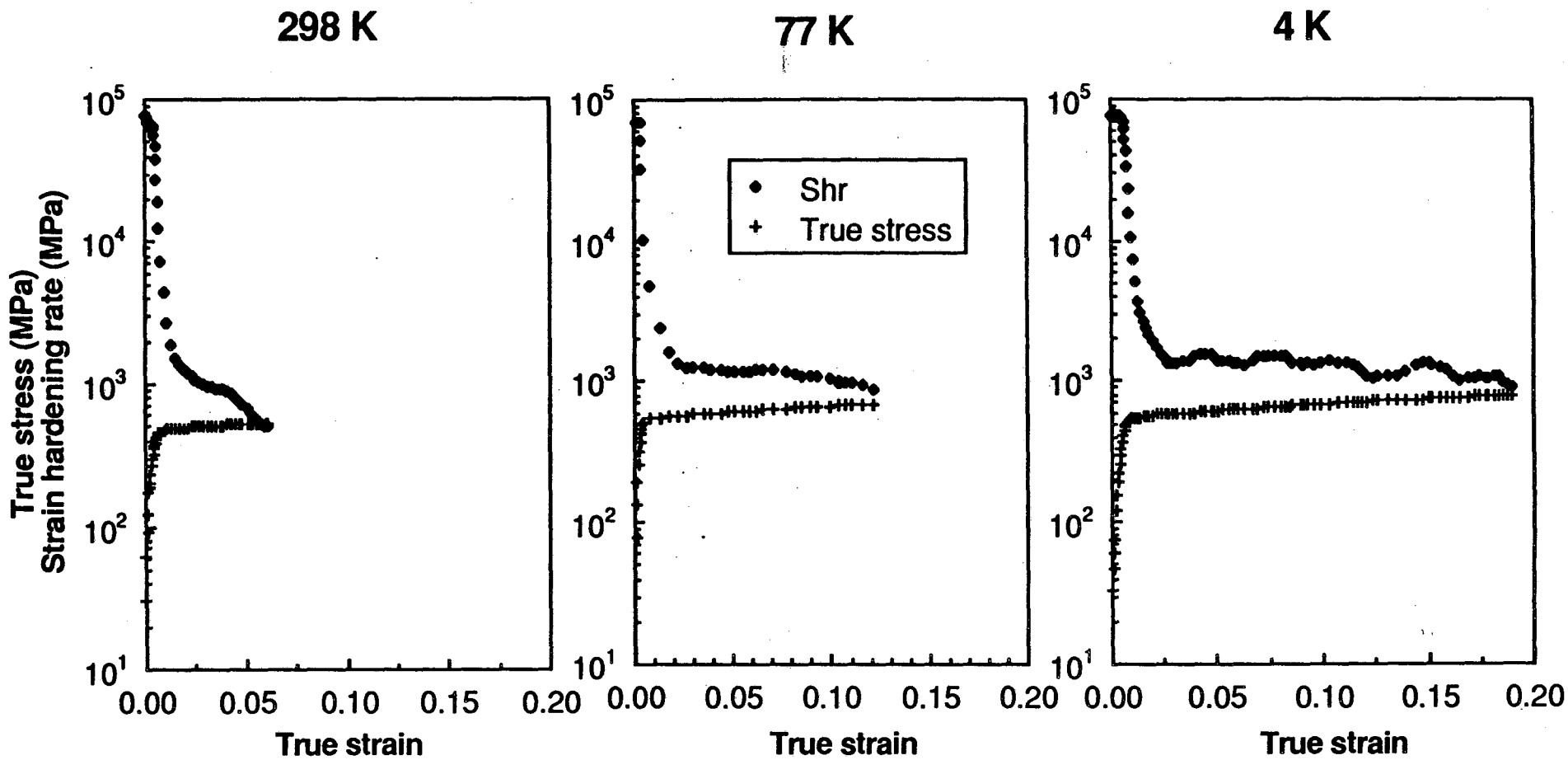
Figure 4. True stress and strain hardening rate (shr) plotted as a function of true strain for alloy 2090-T81 for each test temperature. The true stress and the strain hardening rate (both plotted on the vertical axis) are measured in the same units.
