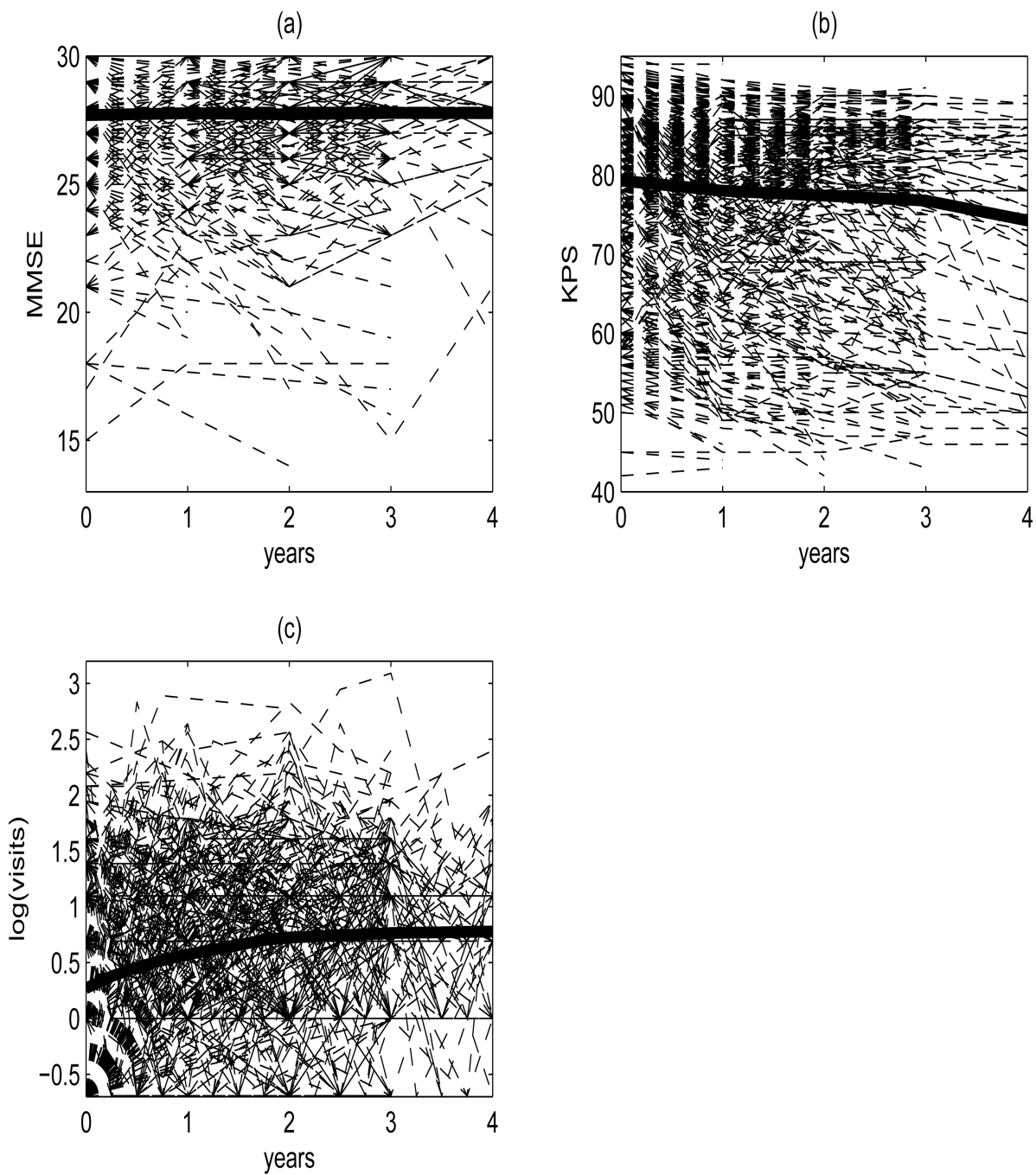
Figure 1. Observed individual trajectories (dashed) and the smoothed estimate of the cross-sectional mean functions (thick solid) for the (a) cognitive impairment score MMSE, (b) physical impairment score KPS and (c) logarithm of the number of clinic visits.
