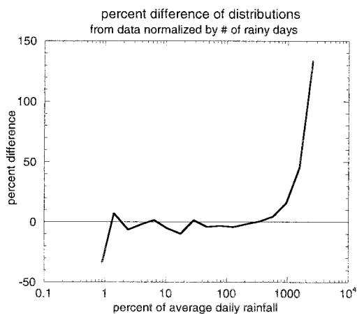
FIG. 6. (a) and (b) As in Fig. 4 except distributions are for Oct–Mar and curves are composite of all years (dotted), composite of six seasons with most (thick) and fewest (thin) events as daily rainfall that exceeds 10% of Oct–Mar climatology. (c) Percent difference of curves (composite of highest minus composite of fewest divided by average) in (b).
