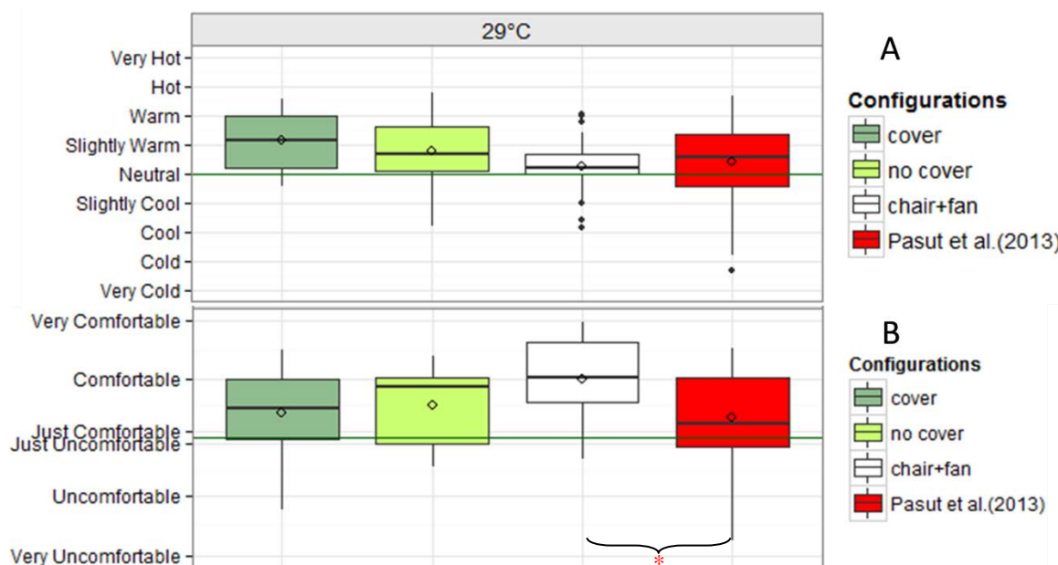
Figure 19A) Whole body thermal sensation, 19B) Whole body thermal comfort
