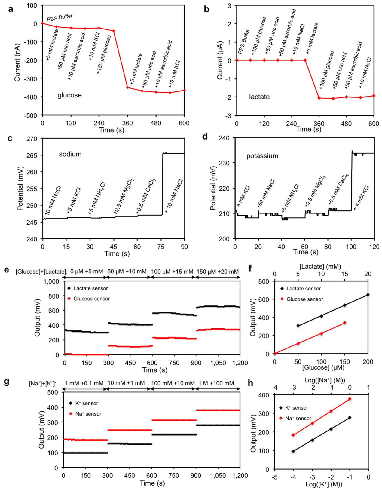
Extended Data Figure 7 | Selectivity study for electrochemical biosensors. a–d , The interference study for individual glucose (a), lactate (b), sodium (c) and potassium (d) sensors using an electrochemical working station. Data recording was paused for 30 s for the addition of each analyte in c and d. e, f , The real-time system-level interference study
