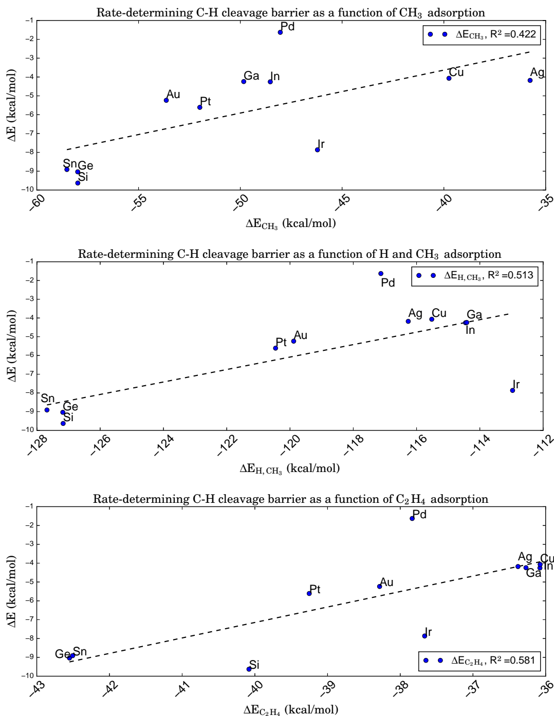
Fig. 8 Brønsted-Evens-Polanyi relation between the adsorption energies of a CH 3 fragment (upper graph), a CH 3 fragment and a single H atom (middle graph), or a C 2 H 4 molecule (lower graph) onto Pt 3 X and the rate-determining first C-H cleavage barrier for the conversion of propane to propene. Despite the 'late' character of the corresponding transition state the assumed correlation to the absorption of the alkyl fragment is very weak. The correlation is slightly improved if a simultaneous adsorption of H and CH 3 at the same site is considered. Surprisingly, the adsorption of C 2 H 4 , the smallest alkene representative, is still better correlated, although the correlation is significantly poorer than was obtained in Fig. 6 based on electronic properties of the clean catalyst.
