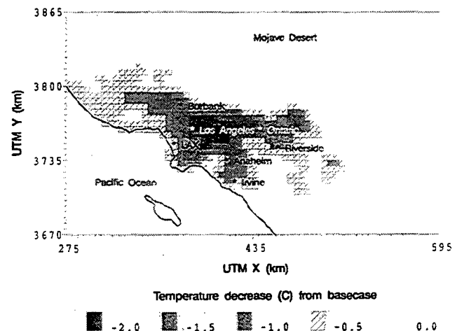
Fig. 2. Impacts of moderate albedo increases on air temperature at 3 p.m. on August 27.
