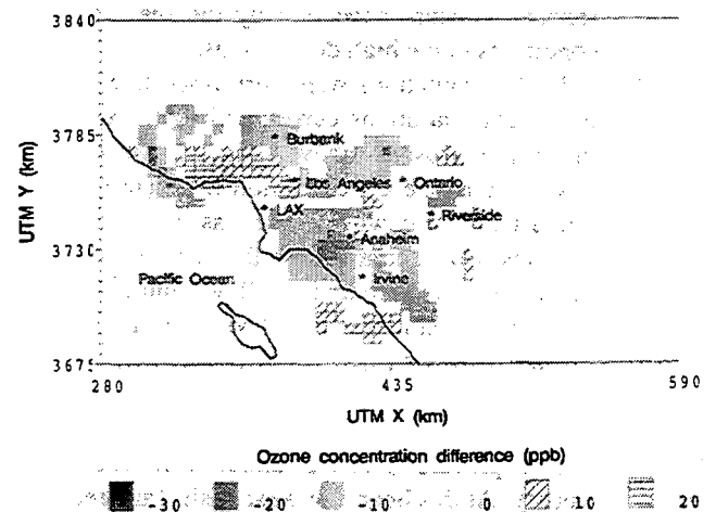
Fig. 3. Deviation in ozone concentrations (ppb) from the base case (at 3 p.m. on August 27) for the moderate albedo increase case.
