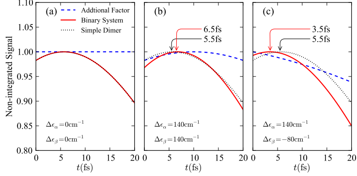
Figure 3: ( Color online) The additional factor \mathcal{A}(\tau, T, t) (blue dashed line), the overall signal |\mathcal{S}^{\text{DN}}(\tau, T, t)|^2 \mathcal{A}(\tau, t) of the binary system shown in Figure 1 (red solid line), and the non-integrated signal |\mathcal{S}(\tau, T, t)|^2 (black dotted line) of the single dimer system for the following sets of parameters \Delta\epsilon_\alpha and \Delta\epsilon_\beta at temperature T_e = 180\text{ K} . (a) \Delta\epsilon_\alpha = \Delta\epsilon_\beta = 0 ; (b) \Delta\epsilon_\alpha = 140\text{ cm}^{-1} and \Delta\epsilon_\beta = 140\text{ cm}^{-1} ; (c) \Delta\epsilon_\alpha = 140\text{ cm}^{-1} and \Delta\epsilon_\beta = -80\text{ cm}^{-1} . In the simulation, we choose we choose different Drude-Lorentian spectral densities for chromophores A and B, with reorganization energies \lambda_A = 60\text{ cm}^{-1} and \lambda_B = 80\text{ cm}^{-1} and cutoff frequencies \omega_{cA} = \omega_{cB} = 50\text{ cm}^{-1} . The inhomogeneous broadenings are \sigma_A = 100\text{ cm}^{-1} and \sigma_B = 50\text{ cm}^{-1} for chromophores A and B respectively. The mean absorption frequencies of chromophores A and B are adjusted to \epsilon_\alpha^0 = 760\text{ nm} and \epsilon_\beta^0 = 800\text{ nm} . The mixing angle \theta is set by using a coupling constant J_0 = 280\text{ cm}^{-1} .
