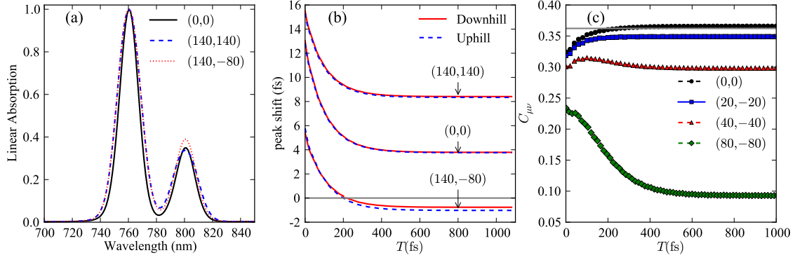
Figure 4: ( Color online) Linear absorption spectra, two-color three-pulse peak shift and coupling coefficient C_{\mu\nu} (see text). (a) linear absorption spectrum with three parameters sets: (1) (\Delta\varepsilon_\alpha, \Delta\varepsilon_\beta) = (0, 0) (solid line); (2) (140\text{cm}^{-1}, 140\text{cm}^{-1}) (blue dashed line); (3) (140\text{cm}^{-1}, -80\text{cm}^{-1}) (red dotted line). (b) Peak shift values for both downhill (red solid line) and uphill (blue dashed line) experiments with the three sets of parameters. (c) Estimated coupling coefficient C_{\mu\nu} as a function of population time T . The exact value C_{\mu\nu} (0.362) is given by the gray solid line. In the simulation, all the other parameters are the same as these in Figure 3.
