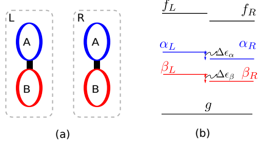
Figure 1: ( Color online) Setup of the system. (a) The binary system with each component as a heterodimer. The two chromophores are marked as A and B . They are coupled with coupling strength J . The indices of components are marked as L and R . Here, we assume no coupling between the chromophores on different components. (b) Exciton (denited by \alpha and \beta for the single excitation states) energy levels diagram. The higher exciton level is shown in blue. Due to the asymmetries between the two components (both in the coupling constants and electronic energy levels), the exciton energy levels are slightly different, and denoted as \Delta\epsilon_\alpha \equiv \epsilon_\alpha^L - \epsilon_\alpha^R and \Delta\epsilon_\beta \equiv \epsilon_\beta^L - \epsilon_\beta^R .
