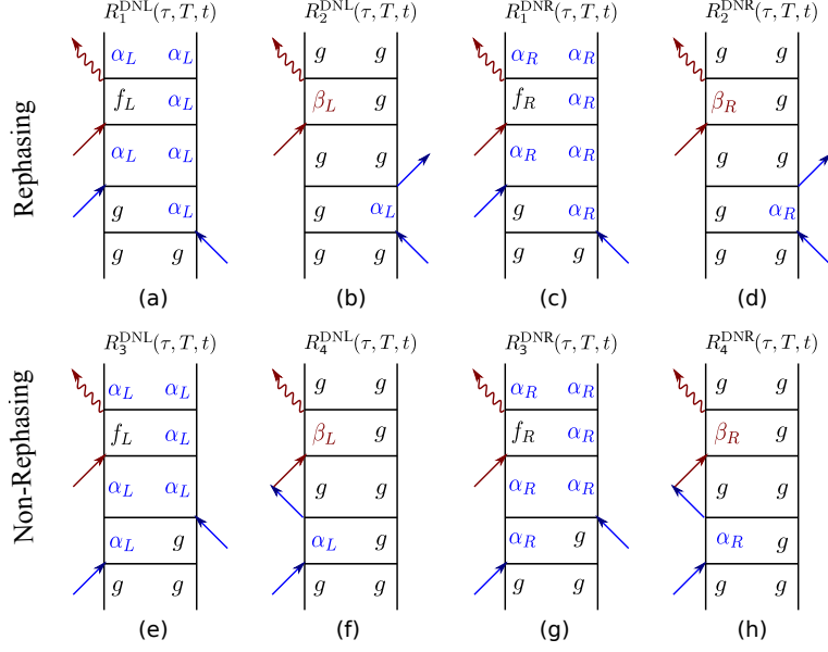
Figure 2: ( Color online) The rephasing and non-rephasing pathways in a downhill two-color peak shift experiment on the binary system. (a-d) The rephasing pathways of the left and right components. (e-h) The non-rephasing pathways of the left and right components. The blue (red) color indicates high (low) frequency of the pulse.
