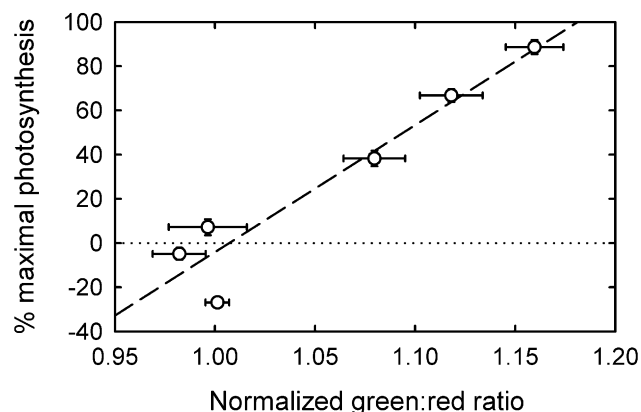
Fig. 5 Percentage of maximal net \text{CO}_2 uptake related to the green : red ratio calculated from images taken in the laboratory simultaneously with gas exchange. Percent net \text{CO}_2 uptake was divided into the six categories: 100% to 75% of maximal, 75% to 50%, 50% to 25%, 25% to 0%, 0% to -25%, and -25% to -50%. Color data were averaged within those categories. Data are mean \pm SE; n = 5 .
