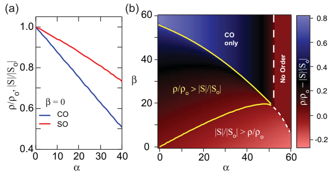
FIG. 4. (a) Calculated normalized amplitude of the CO and SO order parameters when the lattice distortion couples only to the CO. The amplitude for a given \alpha is normalized to the amplitudes when u = 0 , i.e., S_0 and \rho_0 . (b) Stability phase diagram obtained by subtracting the calculated CO and SO amplitudes, i.e., \rho/\rho_0 - |S|/|S_0| , as a function of \alpha and \beta . The region bounded by yellow solid lines is where SO is affected more by the lattice distortions than CO. The values of all the parameters are detailed in the Supplemental Material.
