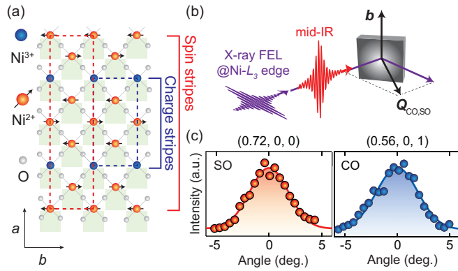
FIG. 1. (a) Stripe phase of \text{La}_{1.75}\text{Sr}_{0.25}\text{NiO}_4 . The blue markers represent the doped holes that form the charge stripe order. The markers with arrows represent the direction of spins at Ni high spin sites ( S = 1 ), which give rise to the spin stripe order. The blue (red) dashed box indicates the period of the charge (spin) order. (b) The experimental setup is sketched in the top panel. (c) Diffraction peak profiles of SO and CO taken by rotating the sample angle (i.e., rocking curve) in the scattering plane under equilibrium conditions (i.e., without laser pumping). The reciprocal positions of the peak position are indicated in the upper horizontal axis. The trajectories of the rocking curves in the reciprocal space are (0.717, 0, -0.15) - (0.72, 0, 0) - (0.717, 0, 0.15) and (0.52, 0, 1.11) - (0.56, 0, 1) - (0.6, 0, 0.88) for SO and CO, respectively.
