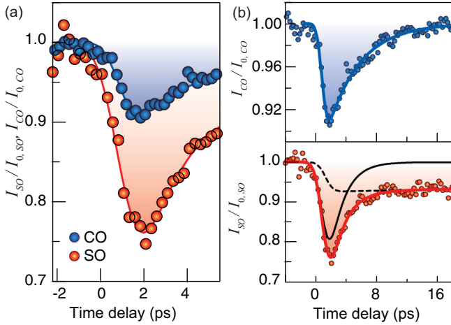
FIG. 3. (a) The response of the SO and CO induced by resonantly exciting the E_u phonons with 14.7 \mu\text{m} laser pulses. Note that the same pump fluence is used for the two measurements. (b) Associated recovery dynamics of SO and CO at longer time. While the dynamics of CO can be described by a single time scale, SO dynamics contains an additional slow time scale, likely associated with spin reorientation [8,22]. The solid curves are single exponential fits of the relaxation time scale. The slow dynamics of SO is fit to a constant offset after time zero.
