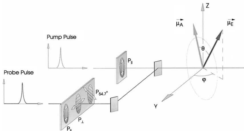
Fig. 14 Implementation of pump-probe polarization measurements. Polarization experiments can be performed by changing the relative orientations of the pump-probe beams from the \parallel/\parallel (parallel-parallel) to \parallel/\perp (parallel-perpendicular) configurations.
