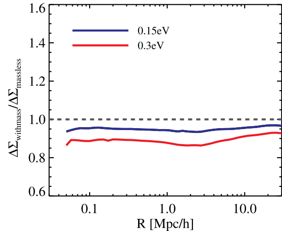
Figure 13. Ratio of \Delta\Sigma from simulations with massive neutrinos to \Delta\Sigma from simulations with massless neutrinos. The blue corresponds to \sum m_\nu = 0.15 eV and the red line corresponds to \sum m_\nu = 0.3 eV. The impact of massive neutrinos leads to a fairly scale independent decrease of \Delta\Sigma over the scales of interest that could partially alleviate the tension reported in this paper.
