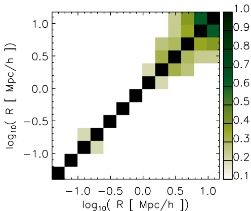
Figure 6. Correlation matrix, \mathbf{C}_{\text{corr}} , computed via bootstrap, smoothed over one pixel scale, and truncated to values greater than 0.2. The outer five data points in our g-g lensing are moderately correlated due to sample variance and correlated shape noise. The inner data points are uncorrelated and the errors on small scales are dominated by shape noise.
