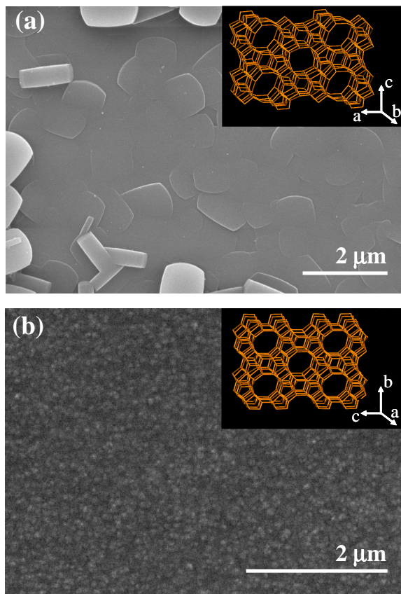
FIGURE 1. SEM Images of (a) in-situ PSZ MFI and (b) spin-on MEL (24 hours) thin films. Loose crystals at the MFI thin film surface were polished away for thermal conductivity measurements. Inserts show (a) the MFI framework viewed down the b -axis, and (b) the MEL framework viewed down the a -axis [26].
