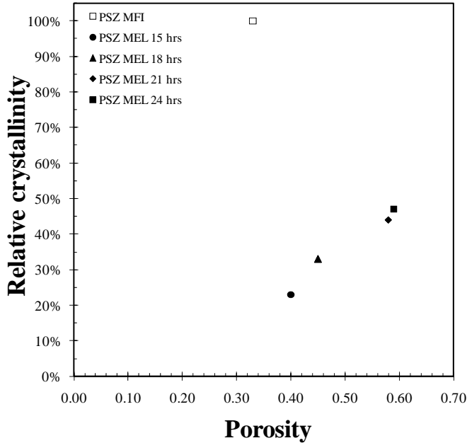
FIGURE 2. Relative crystallinity as a function of porosity for PSZ MEL and MFI thin films [21].
