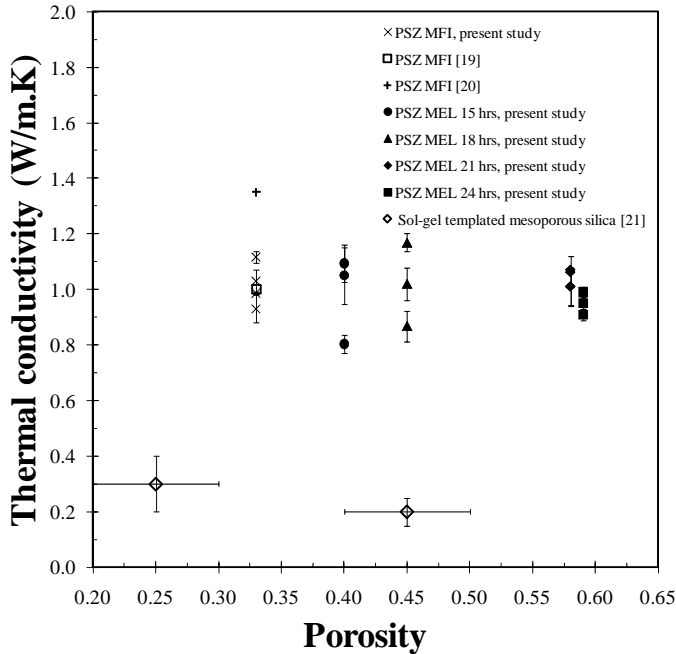
FIGURE 3. Room temperature thermal conductivity of PSZ MEL and MFI thin films as a function of porosity, along with the average thermal conductivity previously reported for MFI films [19, 20] and for templated mesoporous silica thin films [21].
