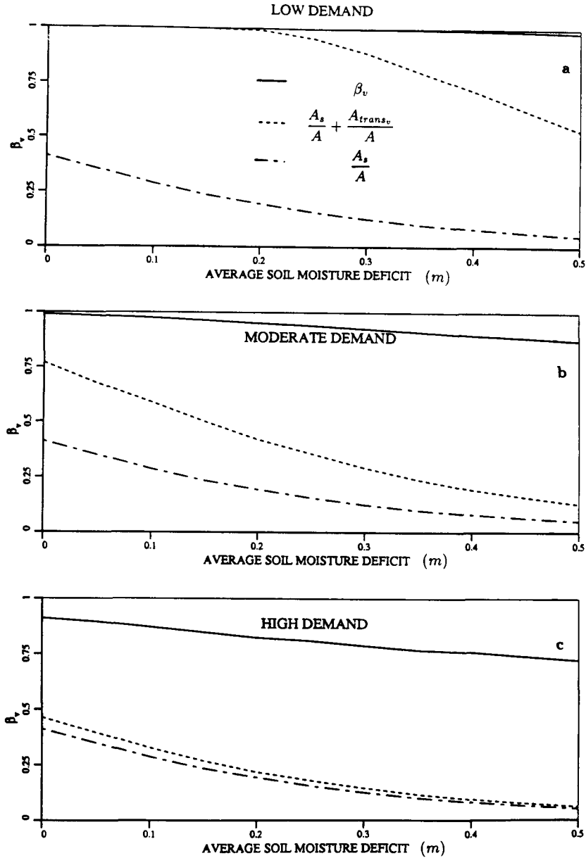
Fig. 4. Transpiration efficiency ( \beta_v ) vs average storage deficit ( \bar{s} ) with potential transpiration equal to (a) 9.0 \times 10^{-6} \text{ m h}^{-1} ; (b) 3.0 \times 10^{-5} \text{ m h}^{-1} ; (c) 3.0 \times 10^{-4} \text{ m h}^{-1} ; \Delta t = 0.25 \text{ hr} .
