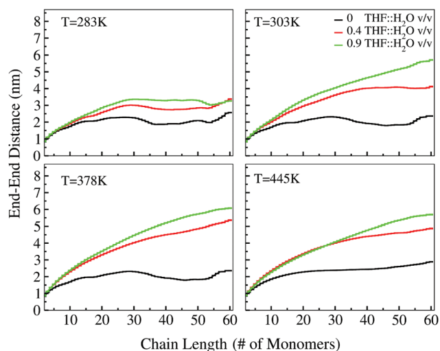
Fig. 5 Lignin end-end (ring) distances versus chain length (in number of monomers). Error bars are standard errors of the mean and are typically of the same size as the width of each line. The same plot projected onto logarithmic axis is provided as ESI Fig. 4.†
