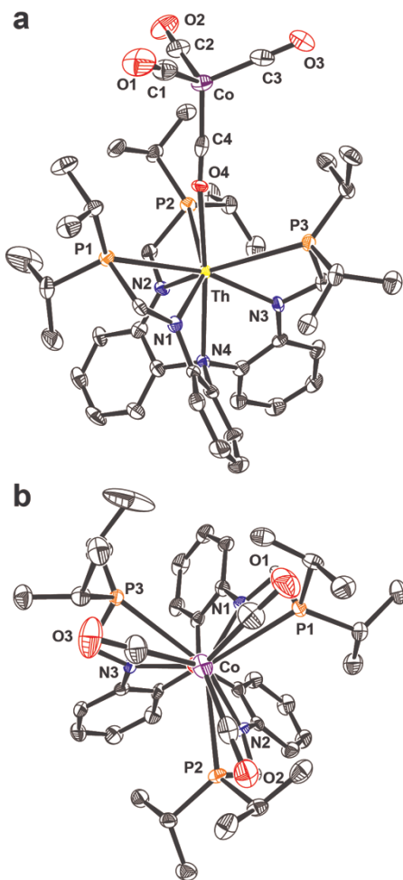
Figure 2. (a) Molecular structure of thorium complex 4 (b) Alternate view of 4 along the Co( \mu -CO)Th axis, illustrating the staggered propeller conformation. Thermal ellipsoids are set to a 50% probability level and hydrogen atoms have been omitted for clarity.
