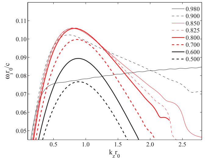
FIG. 4. (Color online) Growth rate vs k_z at different flow speeds (RHD), where v_{z0}/c is labeled above.
