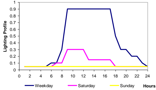
Figure 2. Lighting schedule with occupant sensor control
