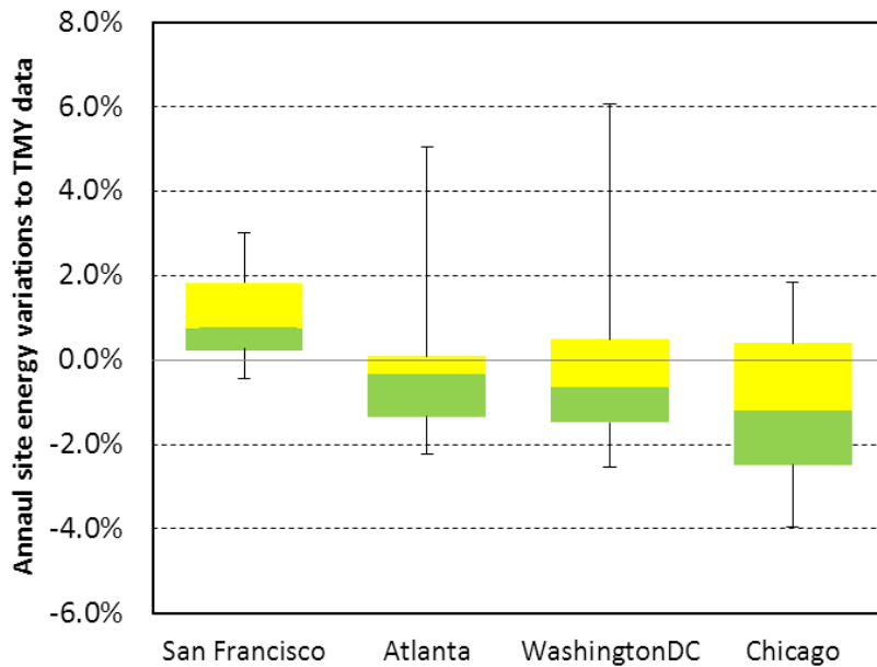
Figure 1. Uncertainties in annual site energy consumption due to actual weather, relative to TMY weather data
