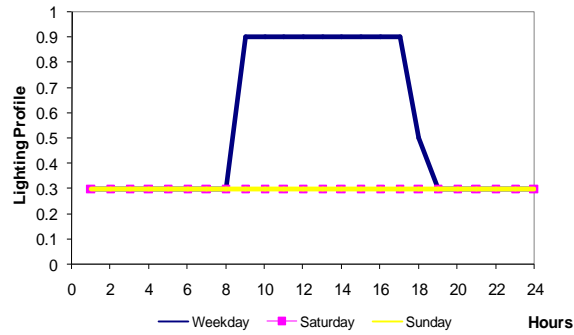
Figure 3. Lighting schedule with manual controls
