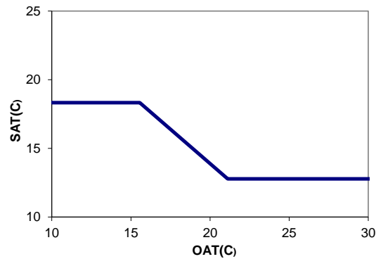
Figure 5. Stepwise function for supply air temperature reset based on outdoor air temperature
