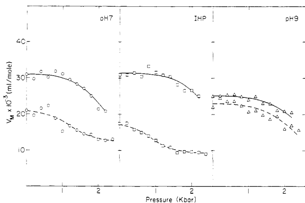
FIGURE 7: Pressure dependence of the average molecular volume calculated from steady-state polarization and average lifetime data using eq 2 for DNS-HB at pH 7 (O), at pH 7 in the presence of 1 mM IHP (□), and at pH 9 (Δ) for 3.2 \times 10^{-5} M (solid lines) and 1.0 \times 10^{-6} M (dashed lines) (in tetramer). Lines do not represent a fit of the data. The buffer was 100 mM Tris-HCl.
