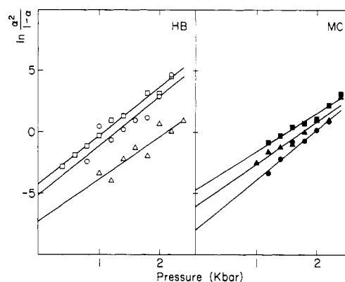
FIGURE 9: Plots of \ln [\alpha^2/(1-\alpha)] vs pressure calculated from the data in Figures 7 and 8 for DNS-HB at 1.0 \times 10^{-6} M tetramer under the three experimental conditions: at pH 7 (O), at pH 7 in the presence of 1 mM IHP (□), and at pH 9 (Δ); and for DNS-MC at 1.0 \times 10^{-6} M tetramer at pH 7 (●), at pH 7 in the presence of IHP (■), and at 4.0 \times 10^{-6} M tetramer at pH 9 (▲). Lines represent linear least-squares regression of the data.
