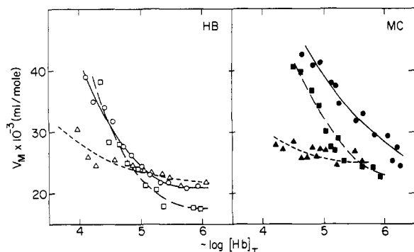
FIGURE 5: Average molecular volumes calculated from the data in Figures 2 and 4 according to eq 2 as a function of -\log [\text{DNS-hemoglobin}]_T in tetramer for DNS-HB at pH 7 (○), at pH 7 in the presence of 1 mM IHP (□), and at pH 9 (△) and for DNS-MC at pH 7 (●), at pH 7 in the presence of 1 mM IHP (■), and at pH 9 (▲). Lines drawn through the points do not represent a fit of the data.
