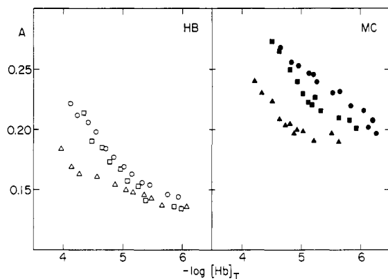
FIGURE 2: Steady-state fluorescence anisotropy as a function of -\log [\text{DNS-hemoglobin}] in tetramer for the standard preparation, HB, at pH 7 (○), at pH 7 in the presence of 1 mM IHP (□), and at pH 9 (△) and for the DEAE major fraction, MC, at pH 7 (●), at pH 7 in the presence of 1 mM IHP (■), and at pH 9 (▲). All buffers were 100 mM Tris-HCl.
