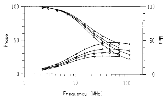
FIGURE 3: Frequency response of DNS-HB fluorescence at pH 7 as a function of protein concentration. Measurements were taken for [(+) phase, (X) mod] 30, [(□) phase, (O) mod] 13, [(△) phase, (Z) mod] 4, and [(*) phase, (◇) mod] 1 \mu\text{M} protein. The buffer was 100 mM Tris-HCl.
