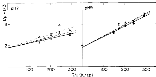
FIGURE 6: Perrin plots for the DNS-MC preparation at pH 7 and pH 9. Three protein concentrations were measured at pH 7: 1.65 \times 10^{-5} M [(◇) and solid line], 1.0 \times 10^{-5} M [(⊗) and dashed line], and 4.0 \times 10^{-6} M [(△) and dotted line (in tetramer)]. At pH 9, the concentrations examined were 2.0 \times 10^{-5} M [(◇) and solid line], 1.0 \times 10^{-5} M [(⊗) and dashed line], and 4.0 \times 10^{-6} M [(▲) and dotted line (in tetramer)]. Aliquots of 60% sucrose were added to the solutions, and background sucrose fluorescence was subtracted using blank containing no protein. Lines represent the result of a linear least-squares reduction of the data.
