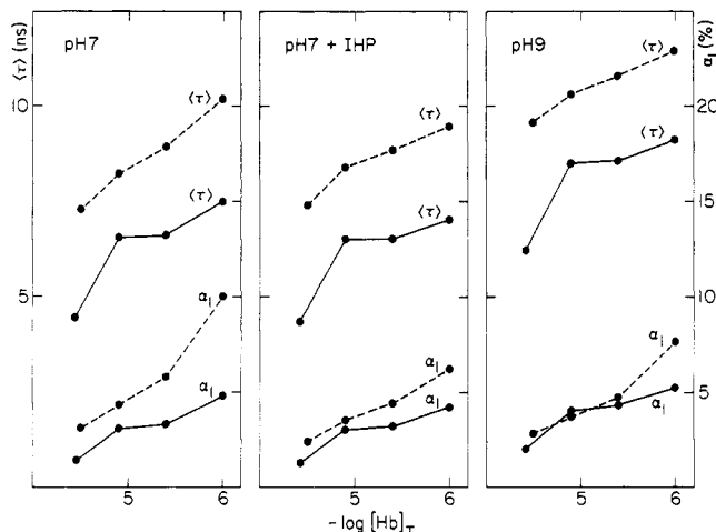
FIGURE 4: Average DNS-hemoglobin lifetime, \langle \tau \rangle , and molecular fraction of the long-lived component ( \alpha_1 ) as a function of protein concentration for the HB preparation (dashed lines) and for the fractionated MC preparation (solid lines) at pH 7, at pH 7 in the presence of 1 mM IHP, and at pH 9. The buffer was 100 mM Tris-HCl.
