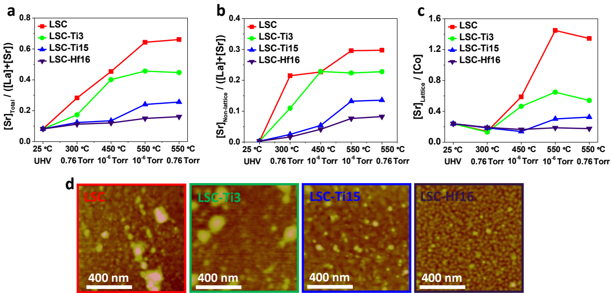
Figure 2. Surface chemical stability on LSC dense thin films. (a) [Sr]_{Total}/([La]+[Sr]) , (b) [Sr]_{Non-lattice}/([La]+[Sr]) , and (c) [Sr]_{lattice}/[Co] ratios at the surface of the LSC and LSC-Me thin films measured in situ at different temperature and oxygen partial pressures by ambient pressure X-ray photoelectron spectroscopy (APXPS). (d) Ex situ atomic force microscopy images of the LSC and LSC-Me films after the APXPS measurements in (a).
