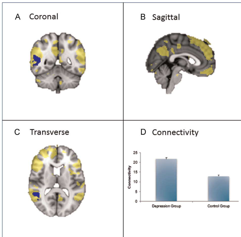
Fig. 1. Default Mode Network engagement in a cross-sectional study of late-life depression as compared to control. This figure shows increased connectivity in the DMN in depression versus control groups ( p < 0.05 , corrected). The blue regions indicate higher connectivity in depression versus control group. The yellow region demonstrates the recruited areas of the DMN. See A–C. The bar graph (D) indicates mean connectivity for depression and control groups. (For interpretation of the references to color in this figure, the reader is referred to the web version of this article.)
