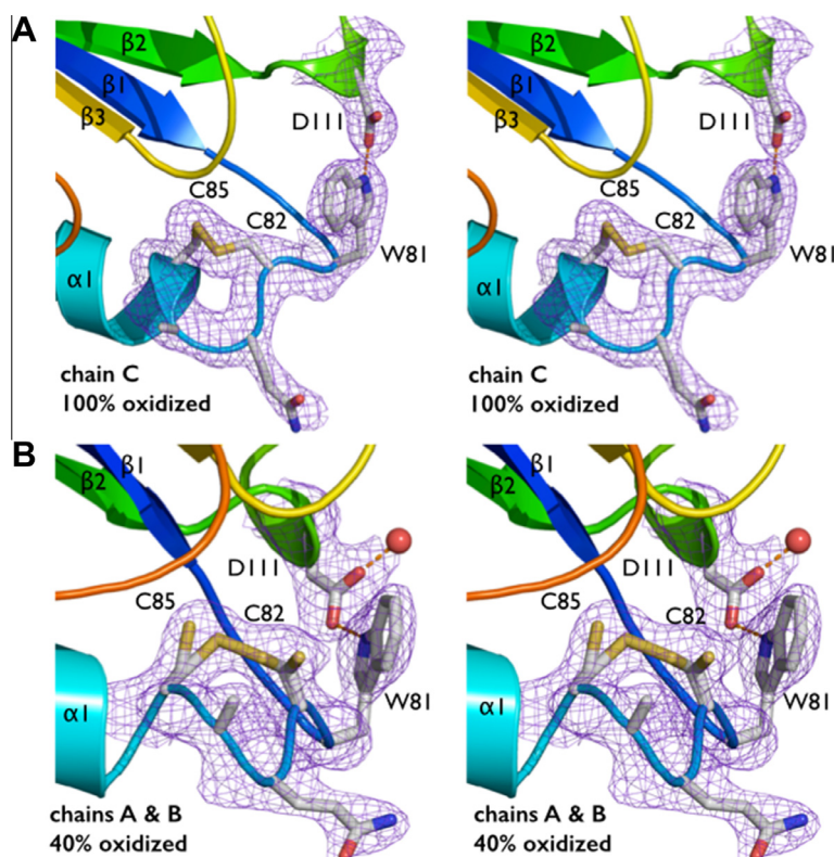
Fig. 2. Plasmodium thioredoxin-2 samples its two redox states in the crystal. 2mFo-DFc Fourier difference electron density maps contoured at 1.5 \sigma showing the catalytic pair of cysteines of Pfal -TRX2 observed in different oxidation states. (A) 100% oxidized form in chain C and (B) 40% oxidized /60% reduced forms in chains A and B. Complete oxidation results in the formation of an intra-molecular disulfide bond. The stabilizing hydrogen bond between conserved residues W81 and D111 is shown.
