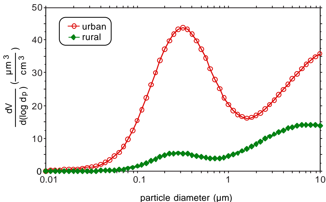
Figure 2. Volume-weighted particle size distribution function for archetypal conditions in ambient urban and rural air. (Source: Seinfeld and Pandis, 1998, Table 7.3)
