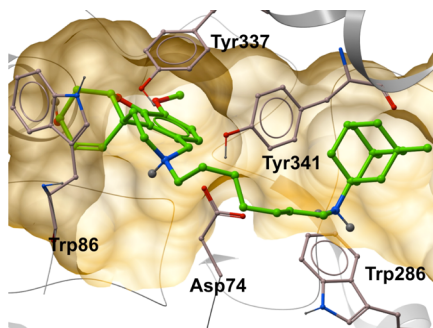
Figure 2. Bound conformation of 6 at the inner and peripheral anionic binding site of human AChE. The inhibitor is displayed in green, while the protein key residues are reported in gray and labeled explicitly. An orange mesh highlights the boundaries of the binding pocket.
