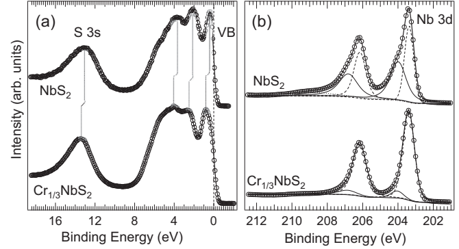
FIG. 9. Comparison of (a) valence band and (b) Nb 3d PES spectra for \text{NbS}_2 (top) and \text{Cr}_{1/3}\text{NbS}_2 (bottom) as measured at normal emission with h\nu = 750 eV. From (a), a comparison of similar features in the VB as well as the shallow S\ 3s core level demonstrates a 0.4 eV shift towards higher binding energy. The suppression of the higher BE peaks of the Nb 3d doublet (solid line) observed in \text{Cr}_{1/3}\text{NbS}_2 is visible in (b).
