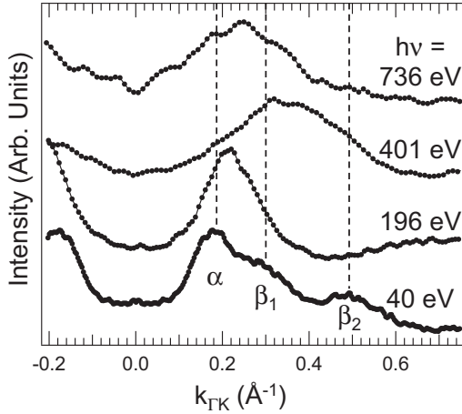
FIG. 8. Direct comparison of MDCs extracted at E_F for h\nu = 40 , 196, 401, and 736 eV depicting k_F crossings about \Gamma . Features from the h\nu = 40 eV spectra are labeled \alpha , \beta_1 , and \beta_2 for the purpose of comparisons. For a description of this notation, see text.
