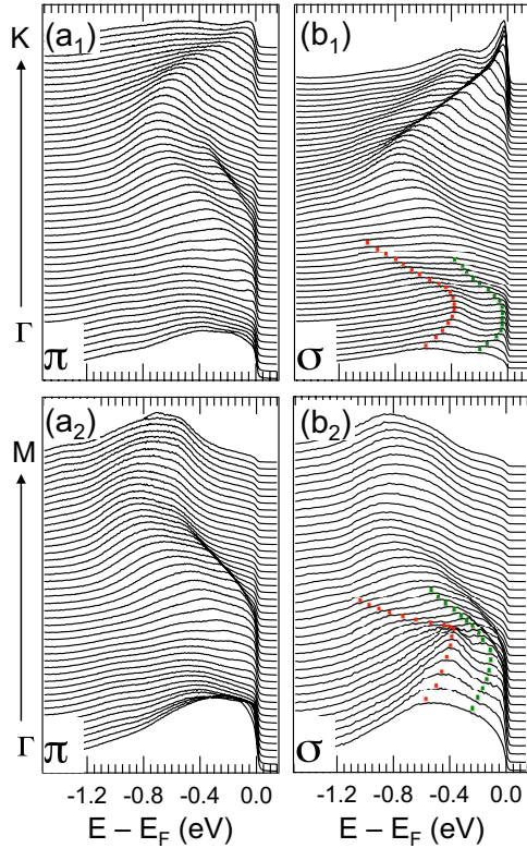
FIG. 17. Stacked EDCs of the corresponding image plots in Fig. 16 shown within \sim 1 eV from E_F . Tick marks tracing the dispersion of the backfolded band (green) and Nb-derived bonding band (red) in (b_1) and (b_2) have been added as a guide to the eye.
