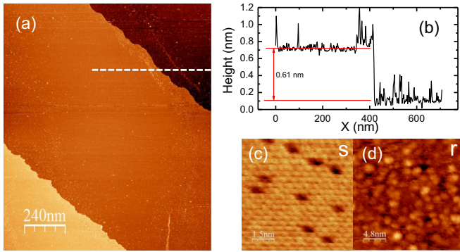
FIG. 2. (a) The STM image of in situ cleaved \text{Cr}_{1/3}\text{NbS}_2 single crystals taken with a bias voltage of -0.4 V illustrating the large-scale surface morphology. (b) Line profile along the broken line in (a) reveals a terrace step height of 0.61 nm with high corrugation near the step edge. (c) and (d) Atomic resolution images of the (c) “smooth” and (d) “rough” areas denoted by s and r, respectively.
