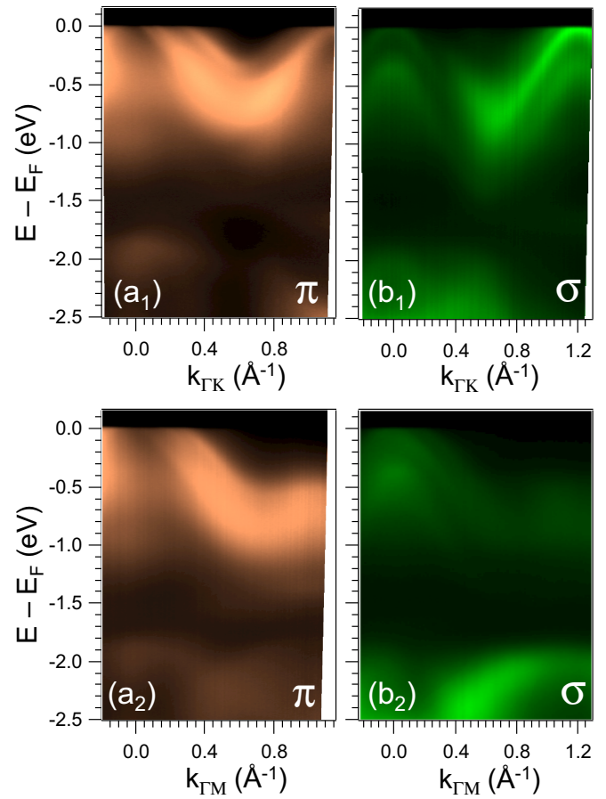
FIG. 16. Band dispersion measured along the ( a_1 and b_1 ) \Gamma K and ( a_2 and b_2 ) \Gamma M direction using \pi -polarized ( a_1 and a_2 ) and \sigma -polarized ( b_1 and b_2 ) photons of energy h\nu = 40 eV.
