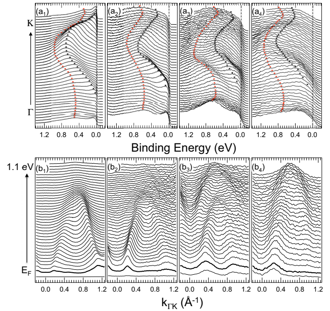
FIG. 7. Stacked EDCs ( a_1 - a_4 ) and MDCs ( b_1 - b_4 ) along the \Gamma K direction extracted from the corresponding image plots depicted in Fig. 6, b_1, b_4 . Tick marks tracing the dispersion of the two bands in proximity to E_F have been added to the EDC stacks in a_1 - a_4 as a guide to the eye. In the MDC stacks, the MDC at E_F is denoted with a thicker line.
