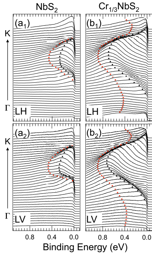
FIG. 12. Stacked EDCs of the corresponding image plots in Fig. 11 shown within \sim 1 eV from E_F . Tick marks tracing the dispersion of the bonding (red) and antibonding (black) bilayer split Nb-bands have been added as a guide to the eye. The Nb-derived bonding band is found to sink \sim 200 meV below E_F (b).
