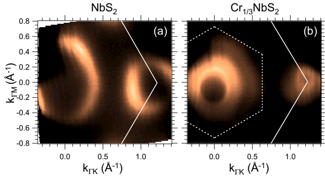
FIG. 10. The FSs of (a) NbS 2 and (b) Cr 1/3 NbS 2 measured along the \Gamma K direction using photons of energy h\nu = 40 eV. The solid and broken lines indicate the 1 \times 1 and \sqrt{3} \times \sqrt{3} BZ, respectively.
