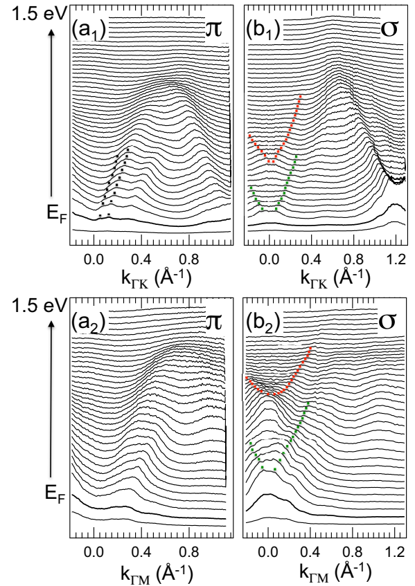
FIG. 18. Stacked MDCs of the corresponding image plots in Fig. 16 shown within \sim 1 eV from E_F . The MDC at E_F are denoted with the thicker line. Tick marks tracing the dispersion of the backfolded band (green) and Nb-derived bonding band (red) in (b_1) and (b_2) have been added as a guide to the eye. Additional tick marks tracing the dispersion of the split \alpha band (black) have been added in (a_1) as a guide to the eye.
