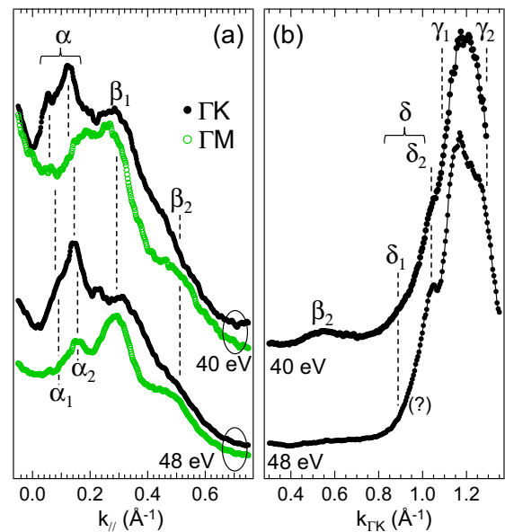
FIG. 23. Direct comparison of MDCs extracted at E_F from Fig. 16 and Fig. 20. The main features of the MDCs are labeled using the same convention as used in Fig. 14.
