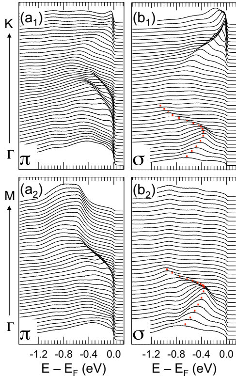
FIG. 21. Stacked EDCs of the corresponding image plots in Fig. 20 shown within \sim 1 eV from E_F . Tick marks tracing the dispersion of the Nb-derived bonding band (red) in (b_1) and (b_2) have been added as a guide to the eye.
