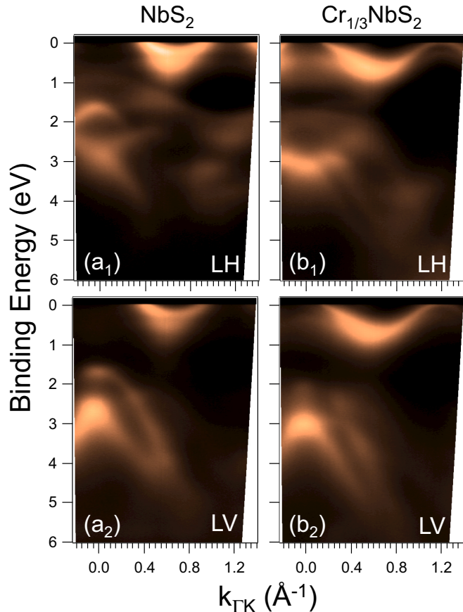
FIG. 11. Band dispersion of (a 1 , a 2 ) NbS 2 and (b 1 , b 2 ) Cr 1/3 NbS 2 measured along the \Gamma K direction over a wide BE range using h\nu = 40 eV photons having a polarization horizontal (a 1 , b 1 ) or vertical (a 2 , b 2 ) with respect to the scattering plane.
