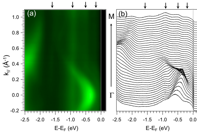
FIG. 4. High resolution ARPES spectra taken from \text{Cr}_{1/3}\text{NbS}_2 with \sigma -polarized photons of energy h\nu = 48 eV. Nondispersive surface states are indicated by arrows in both the (a) image plot and (b) stacked EDCs.
