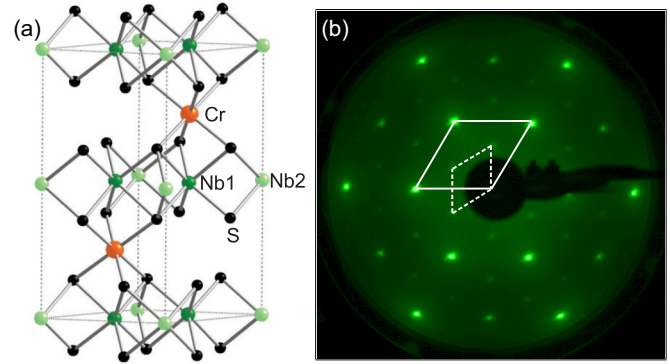
FIG. 3. (a) Unit cell of \text{Cr}_{1/3}\text{NbS}_2 taken from [29]. (b) Representative LEED image obtained from \text{Cr}_{1/3}\text{NbS}_2 with an electron beam energy of 215 eV. The unit cell of the 1 \times 1 (solid) and (\sqrt{3} \times \sqrt{3})R30^\circ (dotted) reciprocal lattice are indicated.
