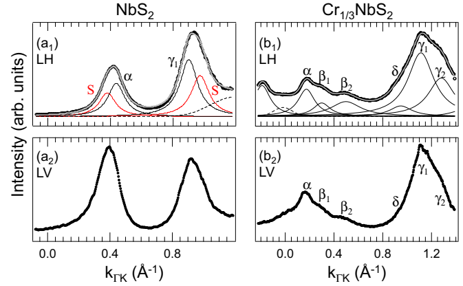
FIG. 14. Direct comparison of MDCs at E_F extracted from the data shown in Fig. 13. In the fit of the MDCs, shown in ( a_1 ) and ( b_1 ), the broken lines denote spectral weight originating from the background. The main features of the MDCs in \text{Cr}_{1/3}\text{NbS}_2 ( b_1 and b_2 ) are likewise denoted in \text{NbS}_2 ( a_1 ). In ( a_1 ), peak S (red) sinks below E_F in \text{Cr}_{1/3}\text{NbS}_2 . A slight misalignment of the sample is responsible for an asymmetry with respect to \Gamma of the MDCs in ( a_2 ) and ( b_2 ).
