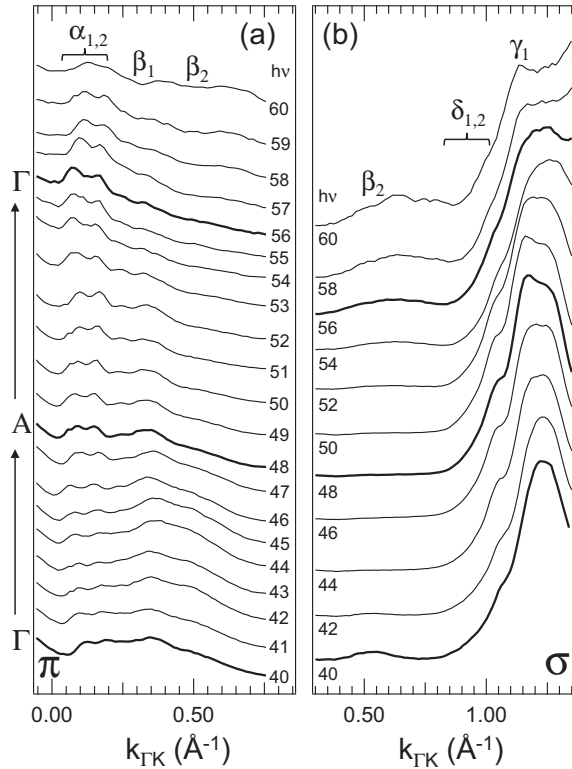
FIG. 24. MDCs extracted at E_F along the \Gamma K direction using (a) \pi -polarized and (b) \sigma -polarized photons. The photon energy was varied from h\nu = 40 eV to h\nu = 60 eV in steps of 1 eV (a) or 2 eV (b).
