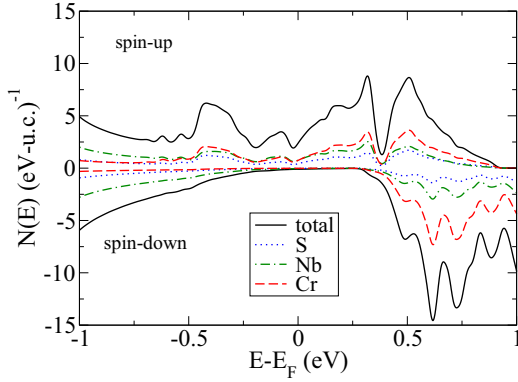
FIG. 25. Calculated spin-polarized DOS of \text{Cr}_{1/3}\text{NbS}_2 in units of inverse electron volts per unit cell. Note the lower values of the DOS for the spin down channel for energies of \sim \pm 250 meV from E_F .
