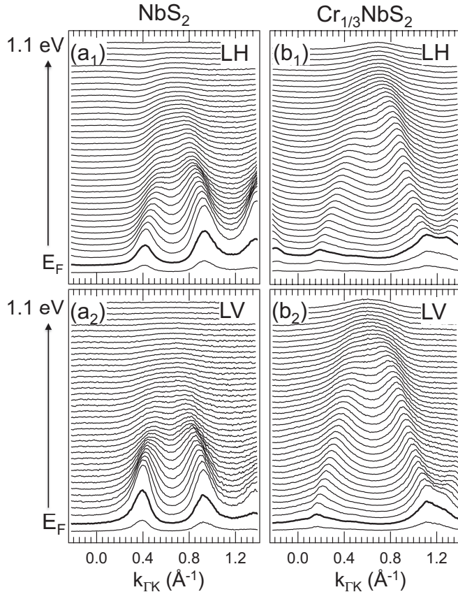
FIG. 13. Stacked MDCs of the corresponding image plots in Fig. 11 shown within \sim 1 eV from E_F . The MDC at E_F is denoted with a thicker line.
