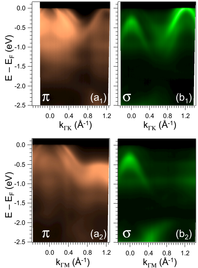
FIG. 20. Band dispersion measured along the (a_1) and (b_1) \Gamma K and (a_2) and (b_2) \Gamma M direction using \pi -polarized (a_1) and (a_2) and \sigma -polarized (b_1) and (b_2) photons of energy h\nu = 48 eV.
