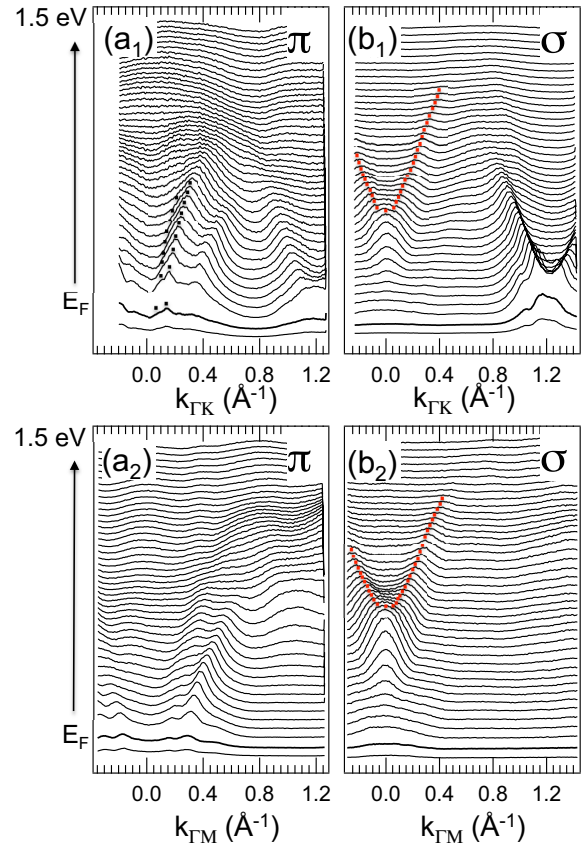
FIG. 22. Stacked MDCs of the corresponding image plots in Fig. 20 shown within \sim 1 eV from E_F . The MDC at E_F are denoted with a thicker line. Tick marks tracing the dispersion of the Nb-derived bonding band (red) in (b_1) and (b_2) and the split \alpha band (black) in (a_1) have been added as a guide to the eye.
