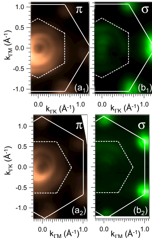
FIG. 15. The FSs of \text{Cr}_{1/3}\text{NbS}_2 measured along the ( a_1 and b_1 ) \Gamma K and ( a_2 and b_2 ) \Gamma M direction using \pi -polarized ( a_1 and a_2 ) and \sigma -polarized ( b_1 and b_2 ) photons of energy h\nu = 40 eV. Solid and broken lines denote the 1 \times 1 and \sqrt{3} \times \sqrt{3} BZ, respectively.
