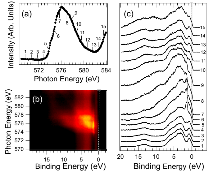
FIG. 5. The ResPES measured from \text{Cr}_{1/3}\text{NbS}_2 across the Cr L_3 absorption edge with photon polarization contained entirely in the sample plane. (a) Cr L_3 XAS measured in total electron yield. (b) ResPES image plot and (c) representative line profiles extracted at the corresponding photon energies labeled in (a).
