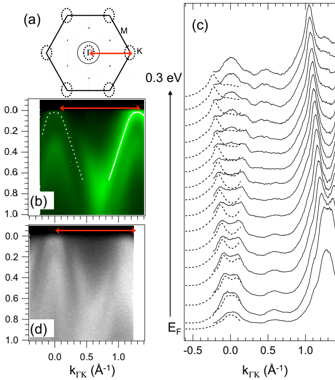
FIG. 19. (a) Sketch of the 1 \times 1 BZ illustrating how the hole-like band at K folds due to a \sqrt{3} \times \sqrt{3} superlattice potential. (b) Band dispersion taken along the \Gamma K direction with \sigma -polarized photons of h\nu = 40 eV. Superimposed on the image plot is a trace of the MDC peak positions of the band at K (solid) translated by a \sqrt{3} \times \sqrt{3} lattice vector (broken line). (c) The MDC stacks having a negative offset taken from 300 meV to E_F from the image plot in (b). Broken lines have been translated by a \sqrt{3} \times \sqrt{3} lattice vector and rescaled so as to directly compare the dispersion. (d) Band dispersion measured along the \Gamma K direction with LV polarized photons of energy h\nu = 196 eV.
