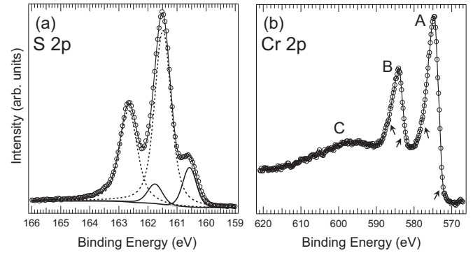
FIG. 1. (a) S2p core level spectrum taken at normal emission from in situ cleaved \text{Cr}_{1/3}\text{NbS}_2 with h\nu = 918 eV. The BE separation between the doublet originating from the surface (solid line) and the deeper layers (dashed line) amounts to \sim 1 eV. (b) \text{Cr}2p core level recorded at normal emission with h\nu = 918 eV. Key features include a spin-orbit split doublet (A and B) and a loss feature (C). The arrows indicate kinks in the line shape of features A and B.
