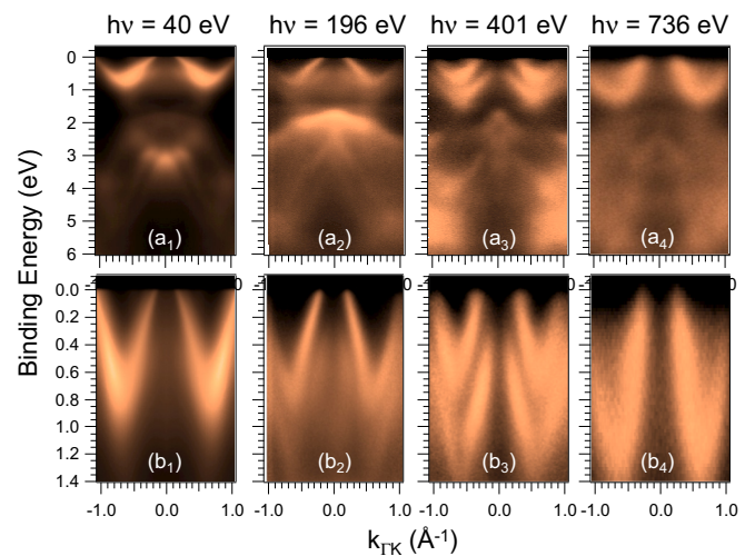
FIG. 6. ARPES spectra measured from \text{Cr}_{1/3}\text{NbS}_2 along the \Gamma K direction over a wide ( a_1 - a_4 ) and narrower ( b_1 - b_4 ) binding energy range using photon energies h\nu = 40 eV ( a_1, b_1 ), h\nu = 196 eV ( a_2, b_2 ), h\nu = 401 eV ( a_3, b_3 ) and h\nu = 736 eV ( a_4, b_4 ). Spectra at h\nu = 40 eV has been symmetrized with respect to the \Gamma point.
