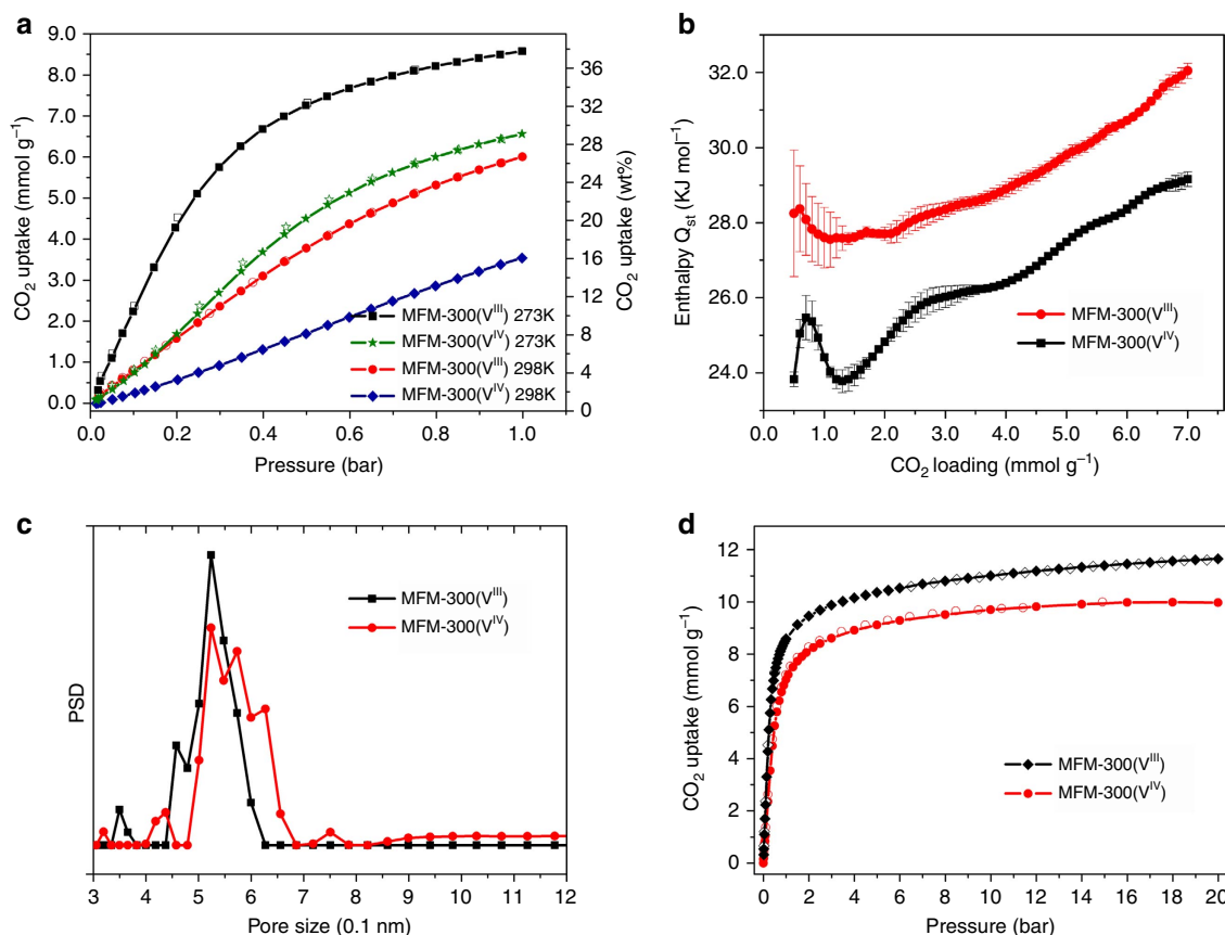
Figure 4 | View of the gas adsorption data. (a) Comparison of the CO 2 adsorption isotherms for MFM-300(VIII) and MFM-300(VIV) at 273 and 298 K and 1.0 bar. (b) Variation of isosteric heat of adsorption Q_{st} as a function of CO 2 uptake for MFM-300(VIII) and MFM-300(VIV) calculated using the van't Hoff isochore on CO 2 adsorption isotherms measured at 273–303 K. Standard deviations are represented by error bars. (c) Comparison of the pore size distribution plots for MFM-300(VIII) and MFM-300(VIV), suggesting a slightly wider pore size in the latter material. (d) Comparison of the CO 2 adsorption isotherms for MFM-300(VIII) and MFM-300(VIV) at 273 K up to 20 bar.
