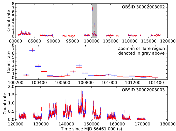
Figure 1. Background-subtracted NuSTAR lightcurves of IGR J17544–2619 OBSID 30002003002 (top panel) and OBSID 30002003003 (bottom panel). The middle panel zooms in on the flare region from OBSID 30002003002. Blue and red plus signs show count rates in 50 s bins for the focal plane modules FPMA and FPMB, respectively. For all panels, the X-axis is time since MJD 56461.0, Y-axes show counts \text{s}^{-1} in the 3–50 keV band. For reference, the average flux in OBSID 30002003003 in the entire 3–50 keV band is (3.53 \pm 0.05) \times 10^{-11} \text{ erg cm}^{-2} \text{ s}^{-1} (1 mCrab).
