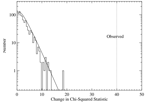
Figure 4. Results of Monte-Carlo simulations for testing line significance for continuum model II (Section 5). We simulated one thousand fake NuSTAR spectra for the continuum-only model ( bodyrad + cut-offpl ), and attempted to fit them with a continuum+line model with N_H fixed at the value obtained with a joint Swift/XRT fit. The solid histogram shows \Delta\chi^2 values obtained in the simulations, and the smooth curve is a \chi^2 distribution with three degrees of freedom. The \Delta\chi^2 attained in actual data (dashed vertical line) is significantly higher than values attained in simulations. This \Delta\chi^2 value differs that in Table 3 due to the simplifying assumptions made in these simulations (Section 5).
