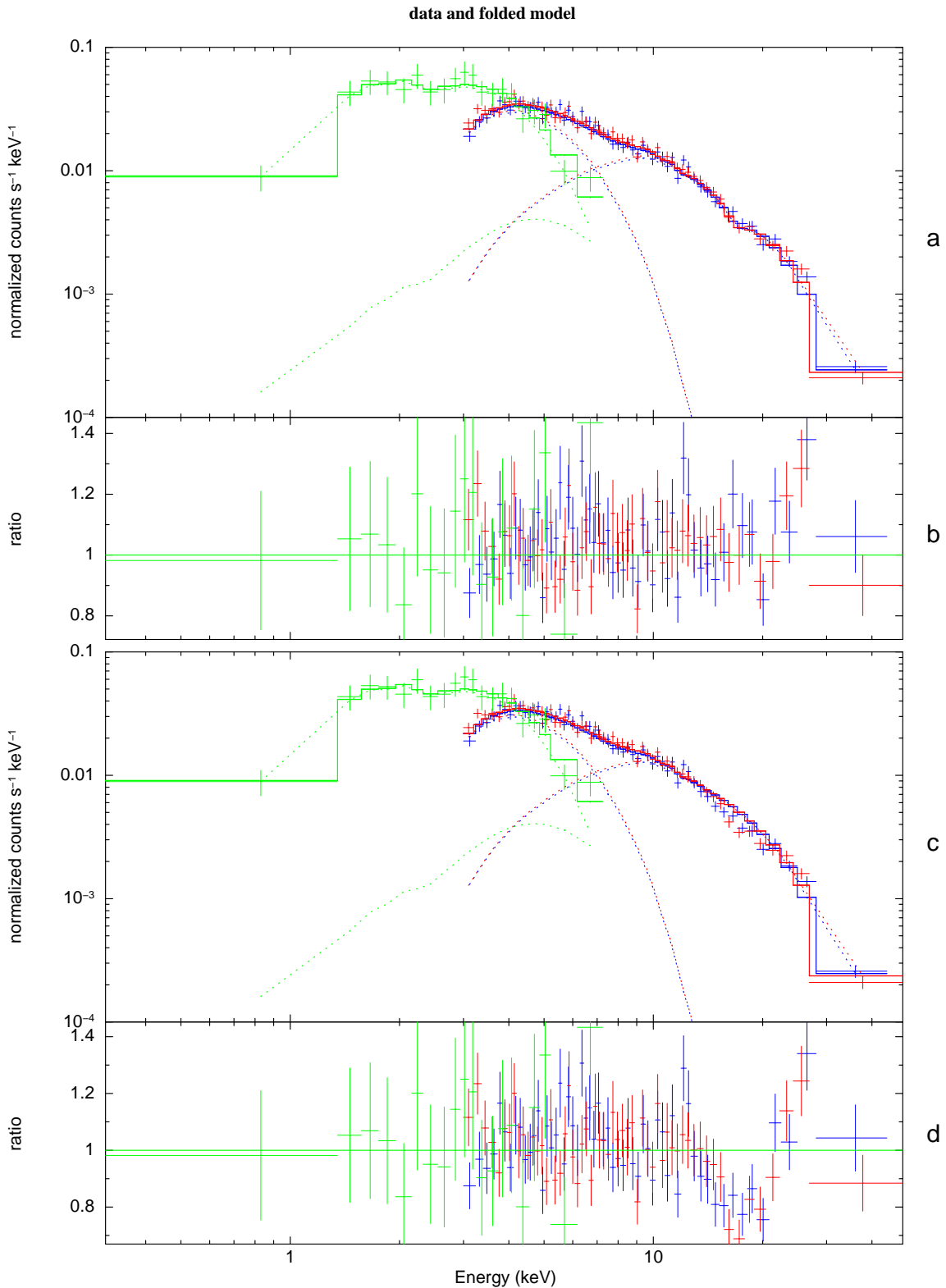
Figure 3. Joint fit to NuSTAR and Swift/XRT data with bbodyrad + nthcomp as the continuum model. Blue, red and green symbols denote data from NuSTAR FPMA, NuSTAR FPMB and Swift/XRT , respectively. For plotting NuSTAR data have been re-binned to a minimum SNR 10 in each bin—actual fitting was done with smaller bins with at least 20 photons each for both: NuSTAR and Swift/XRT . We allow a scaling factor between NuSTAR FPMA, FPMB and Swift/XRT fluxes. Panel a shows the best-fit with the continuum and a single cyclotron line (no harmonics). The ratio data to the model (Panel b) is relatively flat, as expected for a well-fit model. Panel c shows the same model with the cyclotron line deleted (but without refitting). The ratio of data to the model (panel d) clearly show the cyclotron line.
