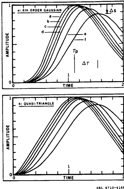
Fig. 1: Output signal pulse shapes for two types of shaper fed by linearly rising signals with different rise times. The upper figure is for a simple 6th order Gaussian while the lower figure is for a quasi-triangular shape. Curves a-f correspond to ratios of rise time/peaking time of 0, .1, .2, .3, .5 and .8.
